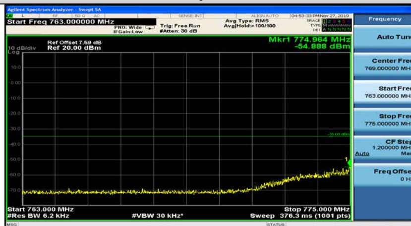
Band13-5MHz-QPSK-23205-12RB#0
