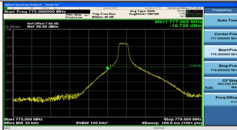
Band13-5MHz-QPSK-23205-1RB#0
