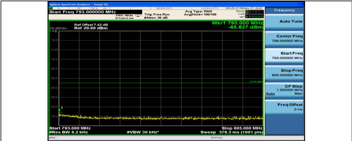
Band13-5MHz-QPSK-23255-25RB#0
