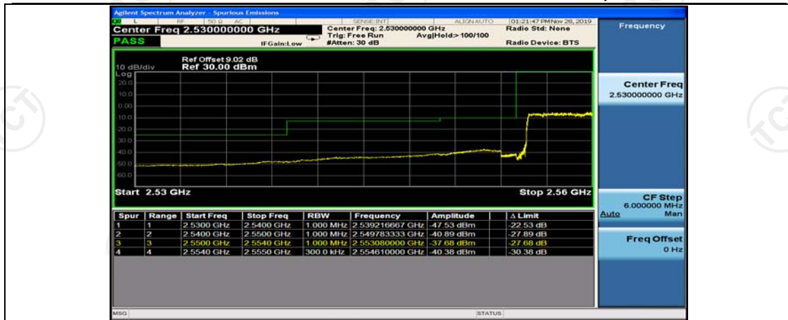
Band41-15MHz-QPSK-41165-1RB#74
