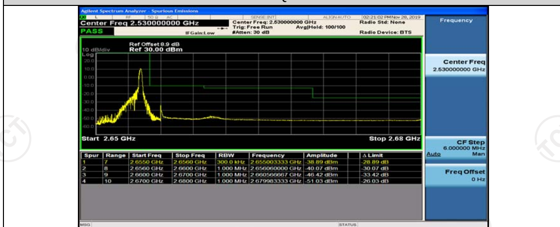
Band41-15MHz-QPSK-41165-75RB#0
