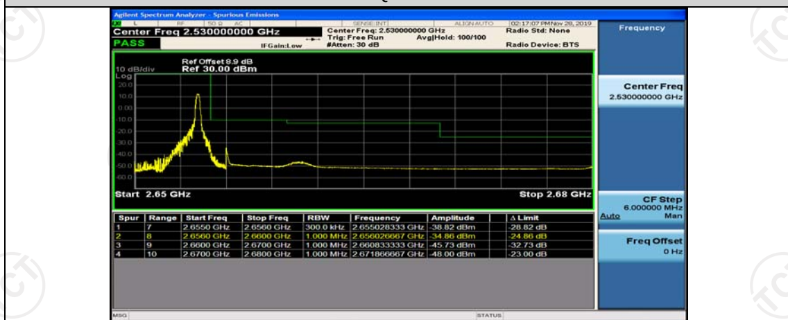
Band41-15MHz-16QAM-41165-1RB#74
