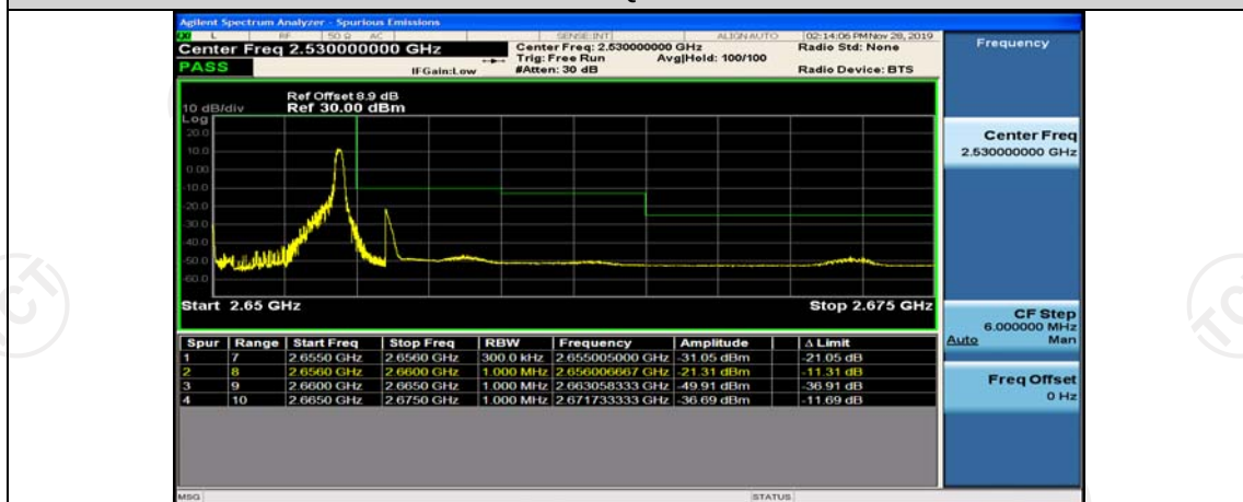
Band41-10MHz-QPSK-41190-50RB#0
