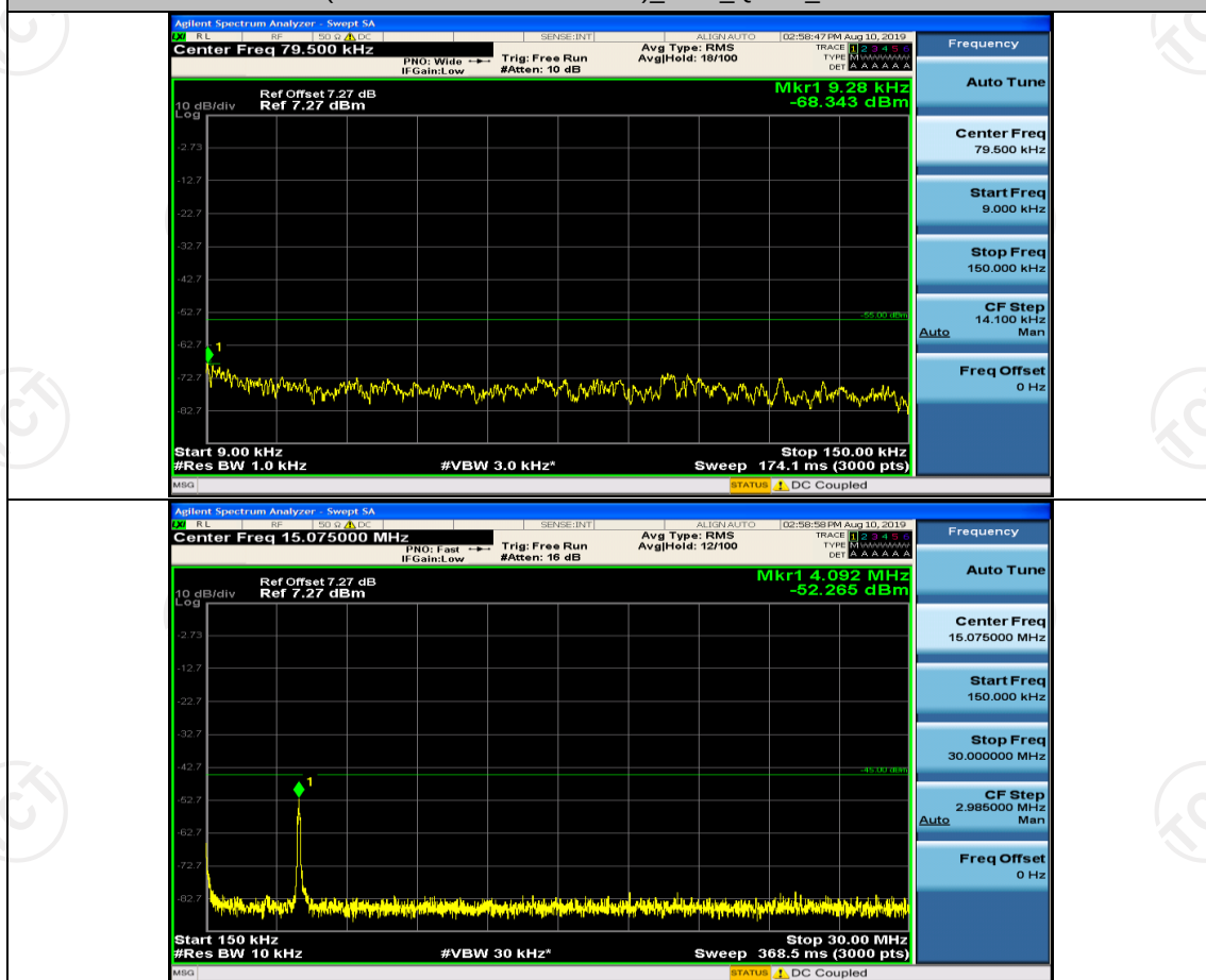
(Channel Bandwidth: 5 MHz)_HCH_QPSK_1RB#0
