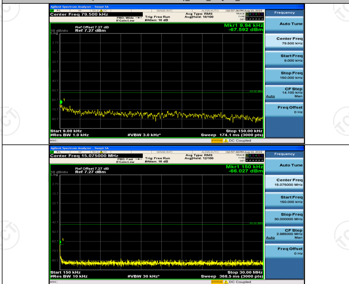
(Channel Bandwidth: 5 MHz)_MCH_16QAM_1RB#0
