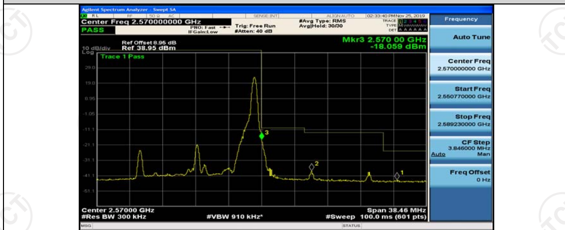
Band7-15MHz-16QAM-21375-75RB#0
