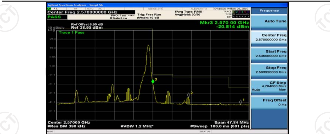
Band7-20MHz-16QAM-21350-50RB#0
