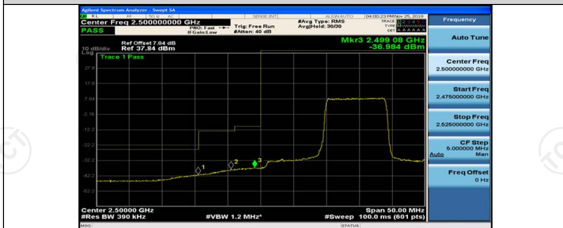
Band7-20MHz-QPSK-20850-50RB#0
