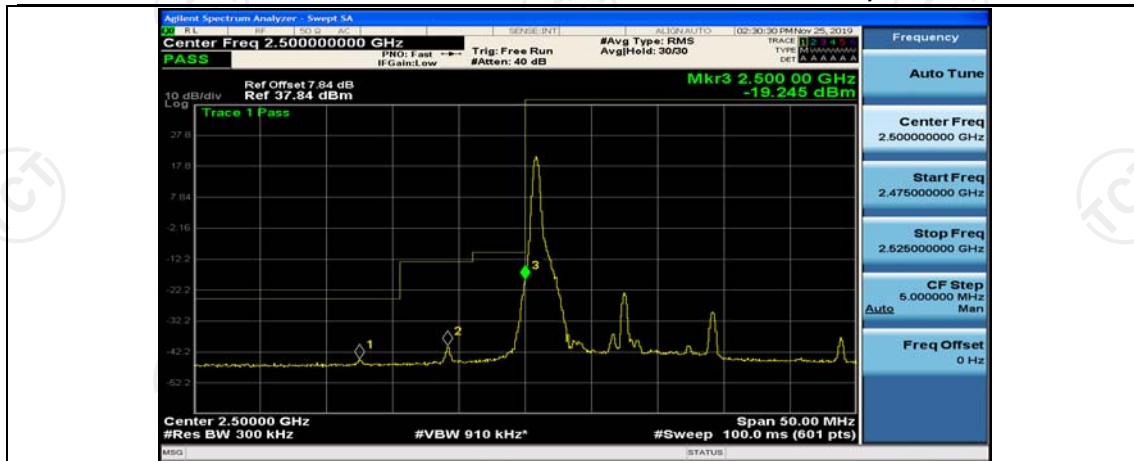
Band7-15MHz-16QAM-20825-38RB#37
