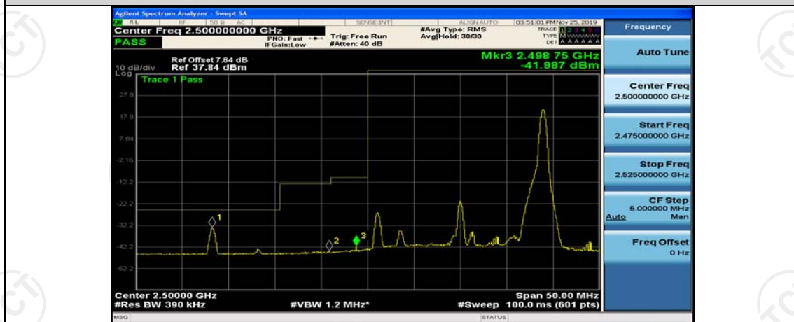
Band7-20MHz-QPSK-20850-50RB#50
