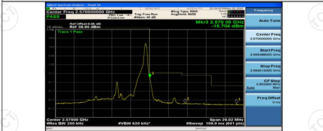
Band7-10MHz-QPSK-21400-1RB#0
