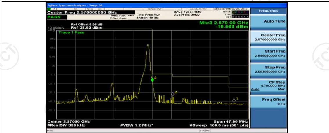
Band7-20MHz-QPSK-21350-50RB#0
