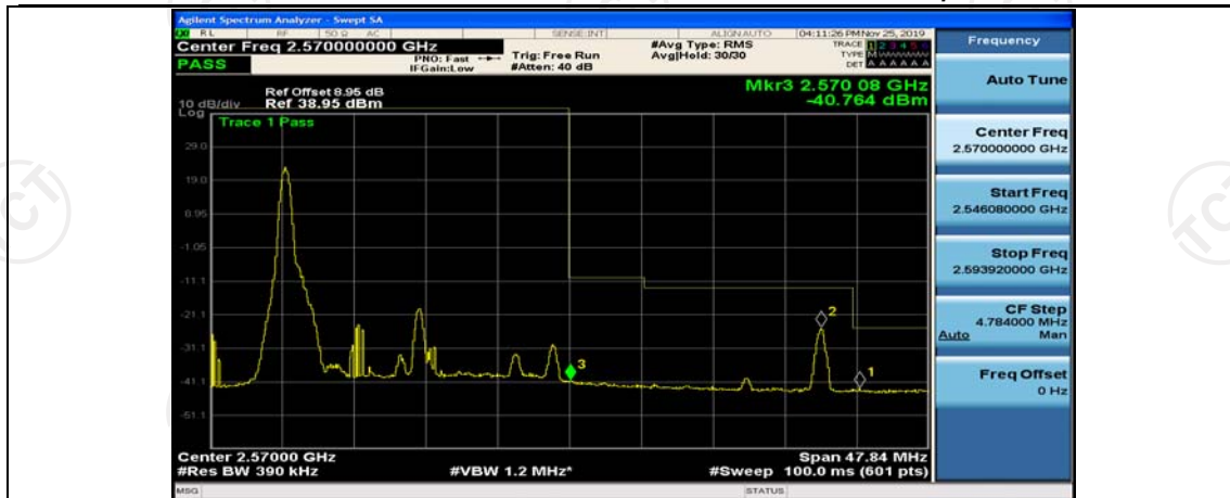
Band7-20MHz-16QAM-21350-1RB#99
