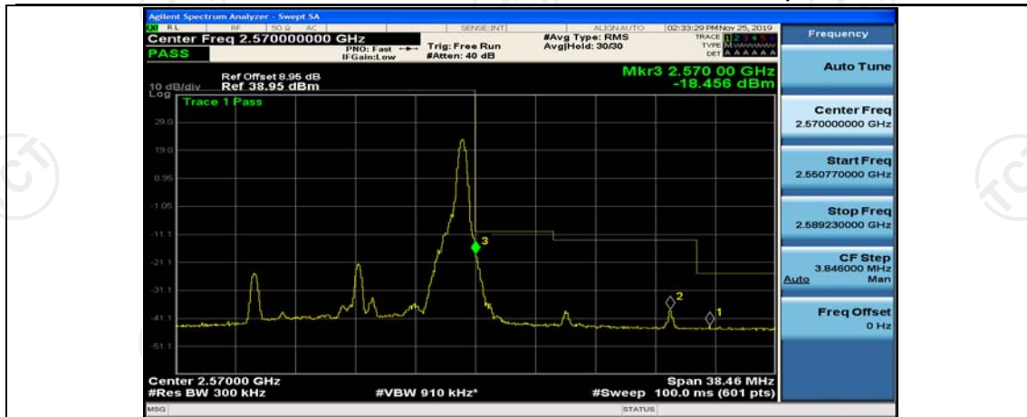
Band7-15MHz-QPSK-21375-75RB#0
