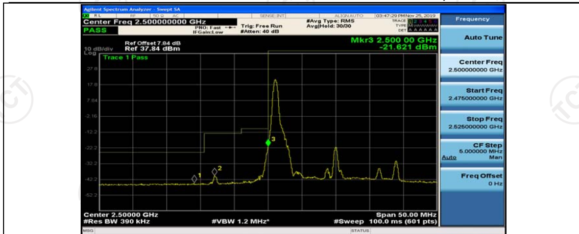
Band7-20MHz-QPSK-20850-1RB#99
