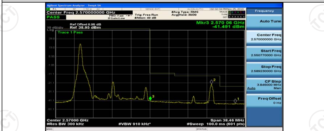
Band7-15MHz-16QAM-21375-1RB#74
