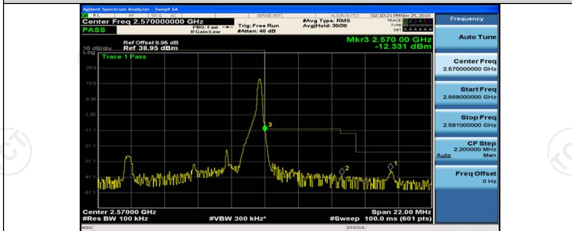
Band7-5MHz-QPSK-21425-1RB#0
