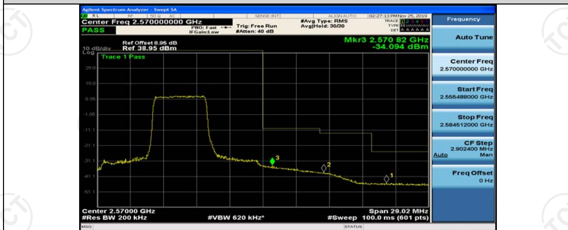
Band7-10MHz-QPSK-21400-50RB#0
