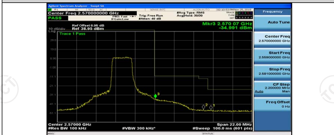
Band7-5MHz-16QAM-21425-12RB#13
