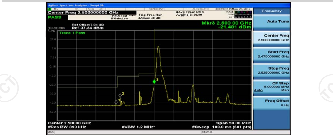
Band7-20MHz-16QAM-20850-50RB#0
