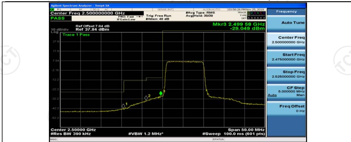
Band7-20MHz-16QAM-20850-50RB#50
