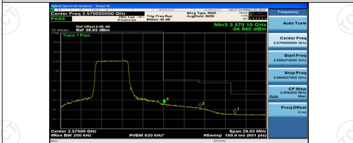
Band7-10MHz-16QAM-21400-25RB#25
