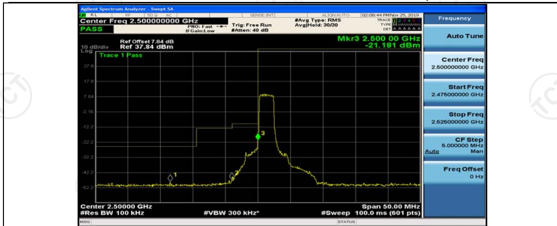
Band7-5MHz-QPSK-20775-25RB#0
