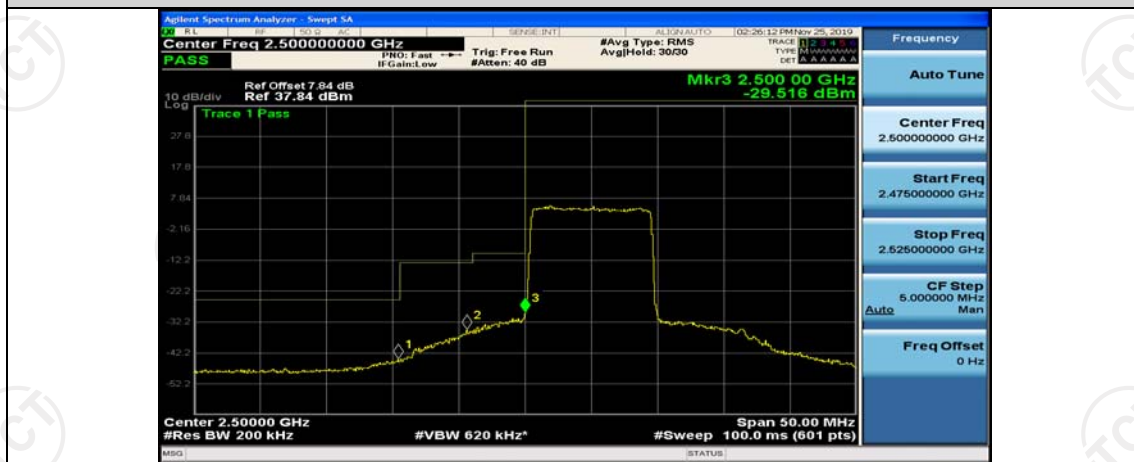
Band7-10MHz-16QAM-21400-1RB#49
