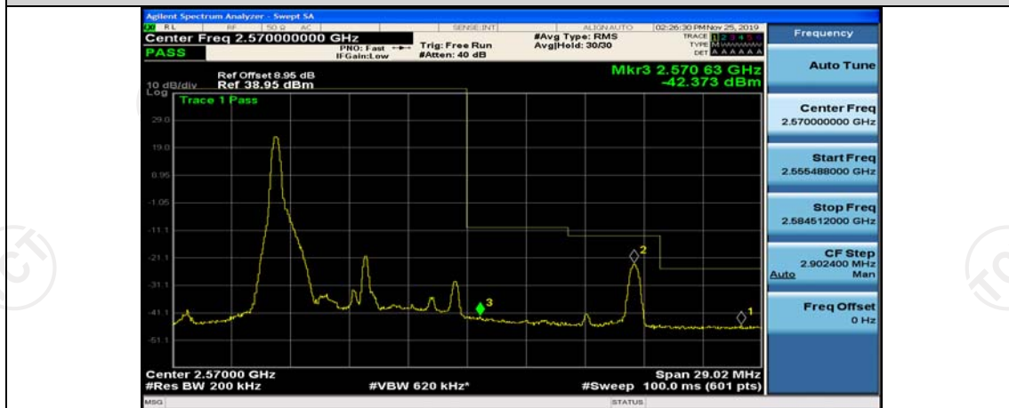
Band7-10MHz-QPSK-21400-25RB#25
