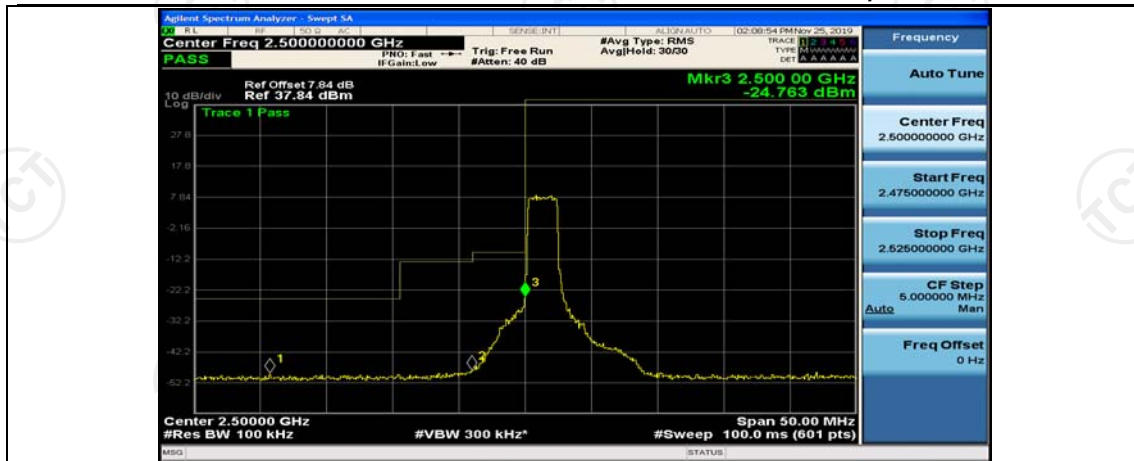
Band7-5MHz-16QAM-20775-12RB#13
