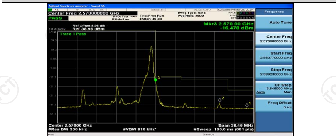
Band7-15MHz-16QAM-21375-38RB#0
