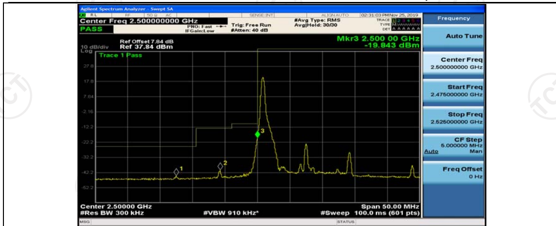
Band7-15MHz-QPSK-20825-38RB#37
