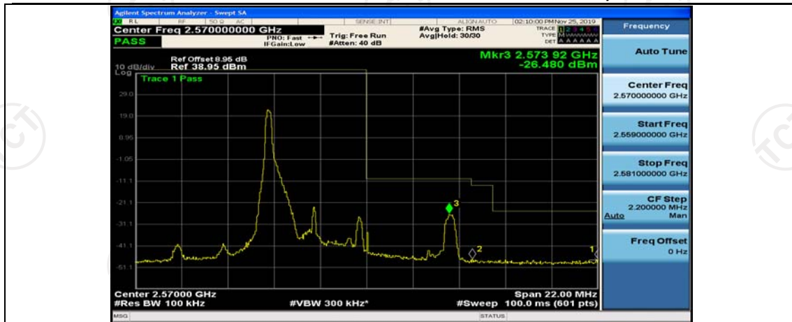
Band7-5MHz-QPSK-21425-12RB#0
