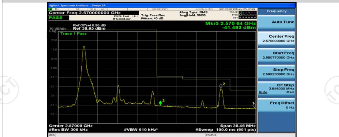
Band7-15MHz-QPSK-21375-38RB#37
