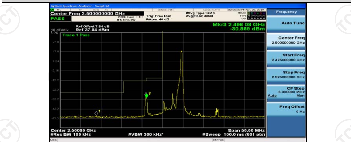
Band7-5MHz-16QAM-20775-1RB#0
