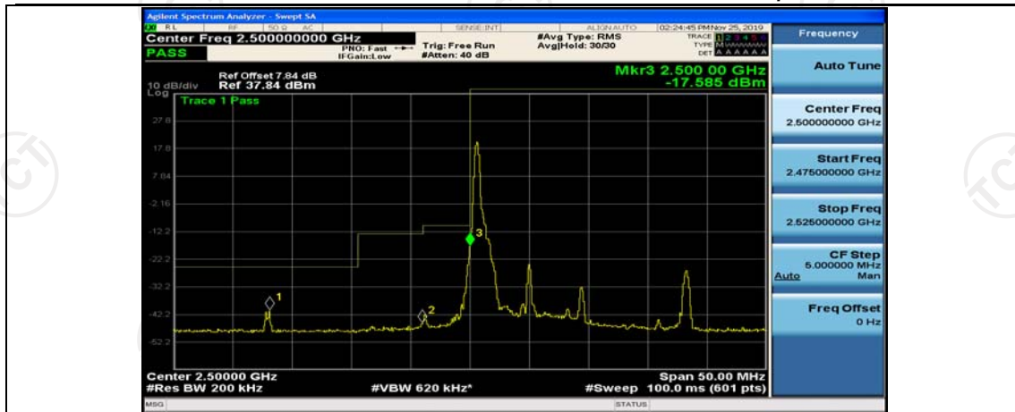
Band7-10MHz-16QAM-20800-1RB#49
