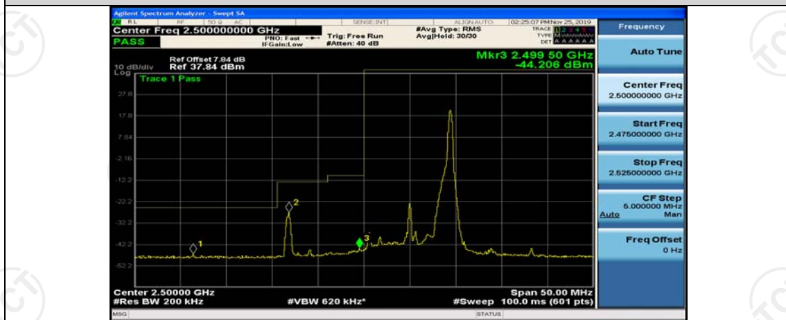
Band7-10MHz-16QAM-20800-25RB#0
