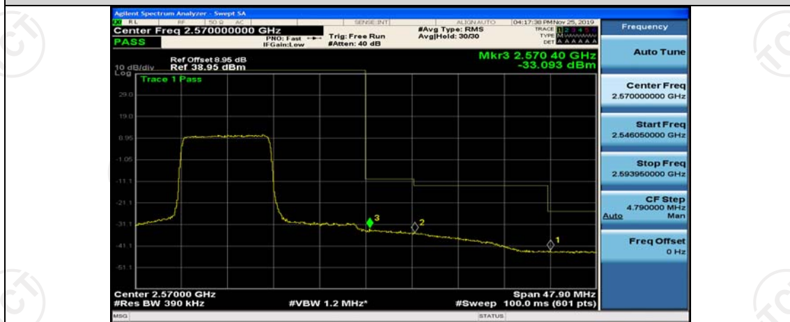
Band7-20MHz-QPSK-21350-50RB#50
