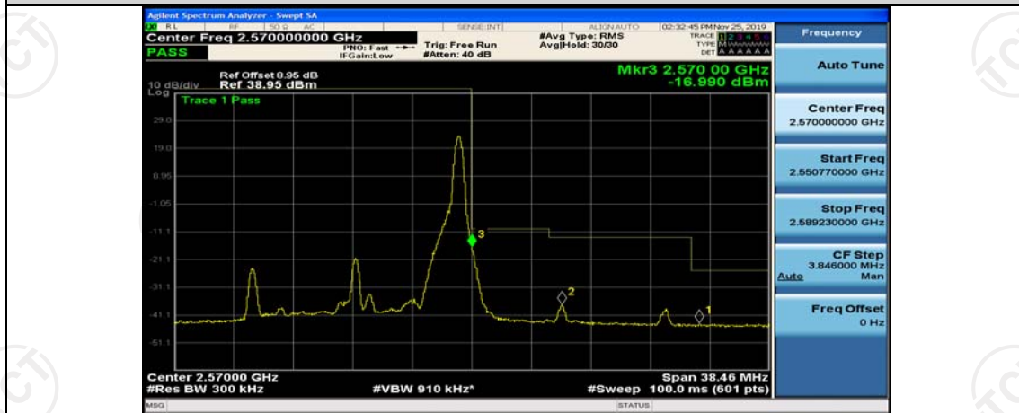
Band7-15MHz-QPSK-21375-38RB#0
