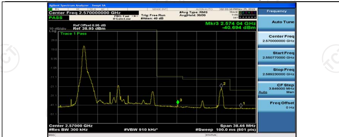
Band7-15MHz-16QAM-21375-38RB#37
