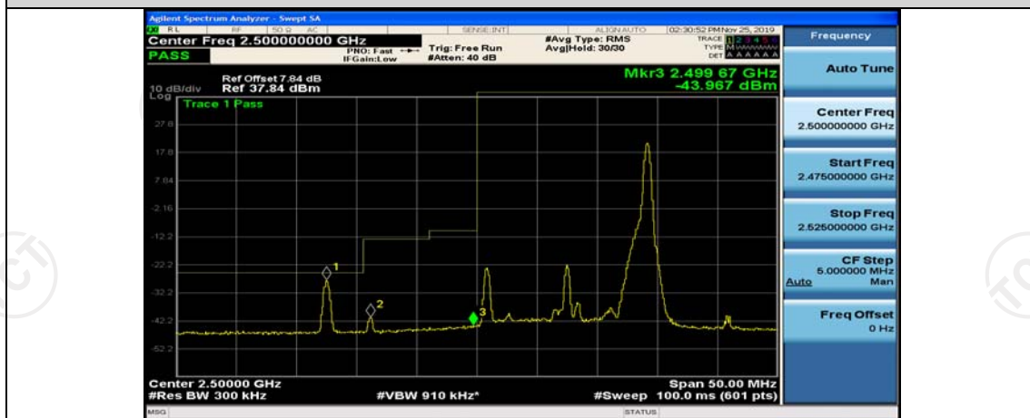
Band7-15MHz-16QAM-20825-1RB#0
