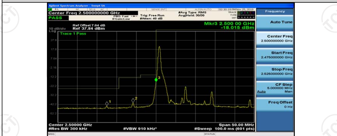
Band7-15MHz-QPSK-20825-1RB#74
