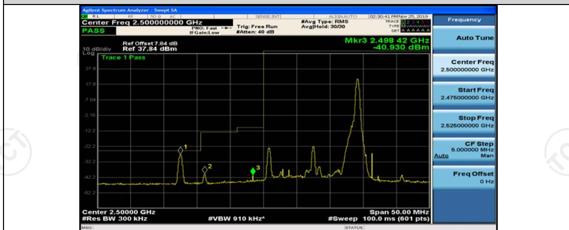
Band7-15MHz-QPSK-20825-38RB#0
