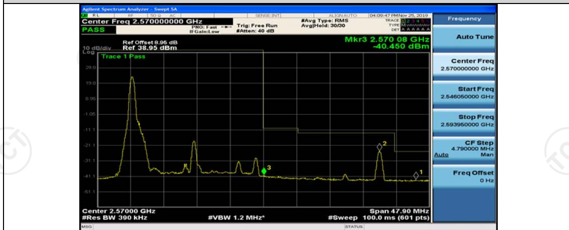
Band7-20MHz-QPSK-21350-1RB#99
