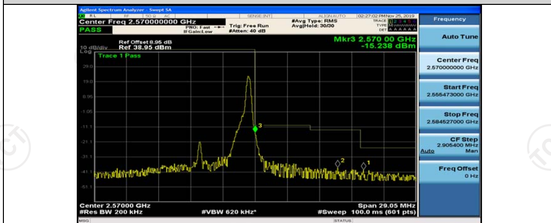
Band7-10MHz-16QAM-21400-1RB#0
