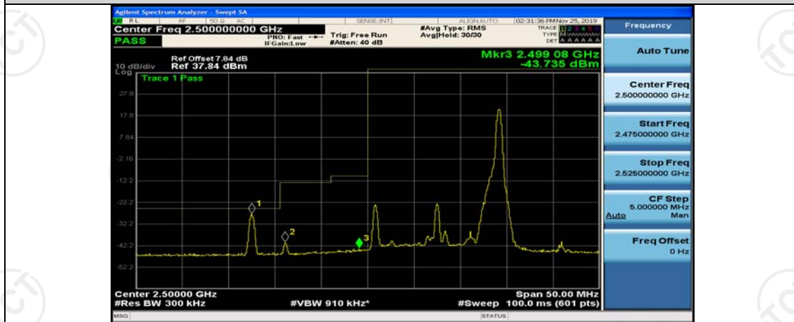
Band7-15MHz-16QAM-20825-38RB#0
