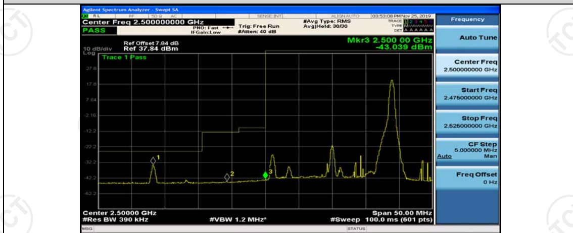
Band7-20MHz-16QAM-20850-1RB#0
