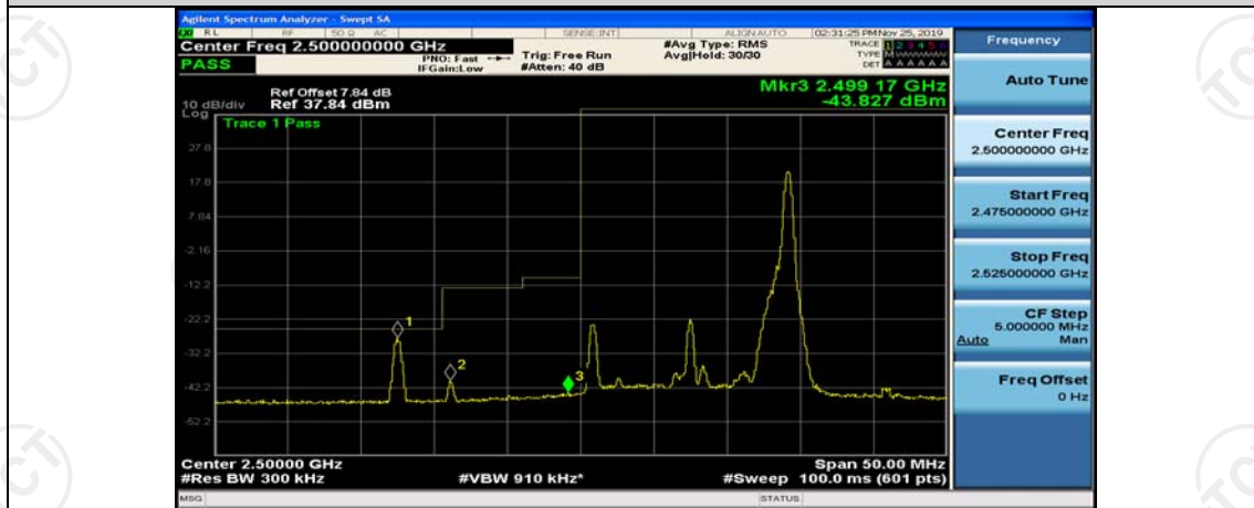
Band7-15MHz-QPSK-20825-75RB#0
