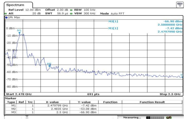
CH39-Bandedge
