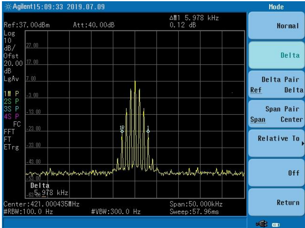
Figure 60. Input 421 MHz @ 6.25 kHz
