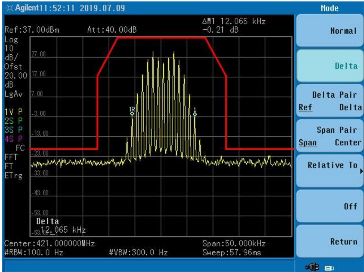
Figure 68. 421 MHz @ 12.5 kHz, Mask D
