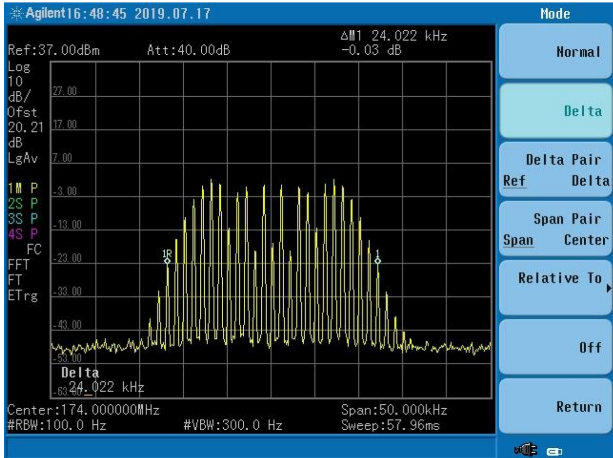
Figure 48. Input 174 MHz @ 25 kHz
