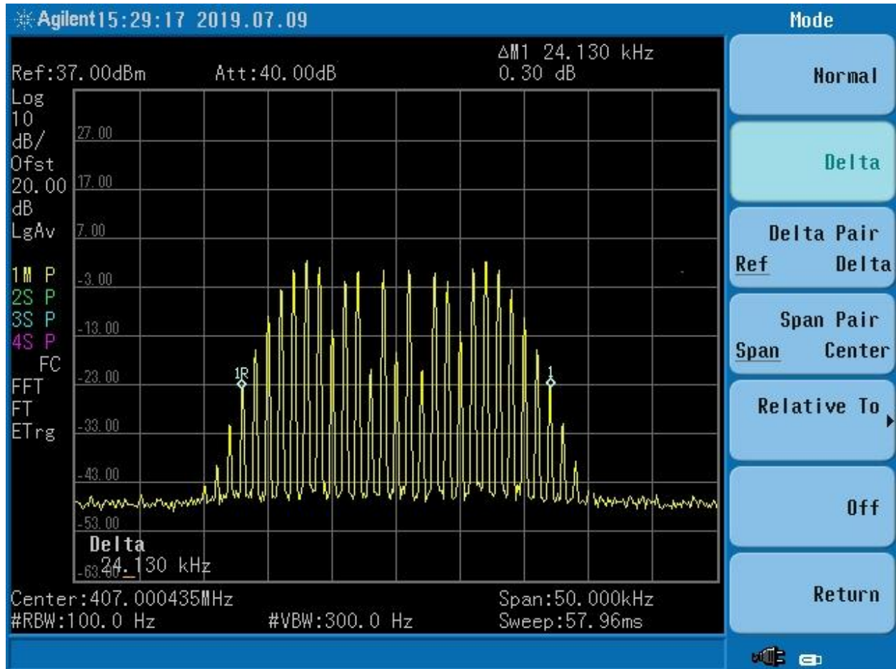
Figure 57. Input 407 MHz @ 25 kHz
