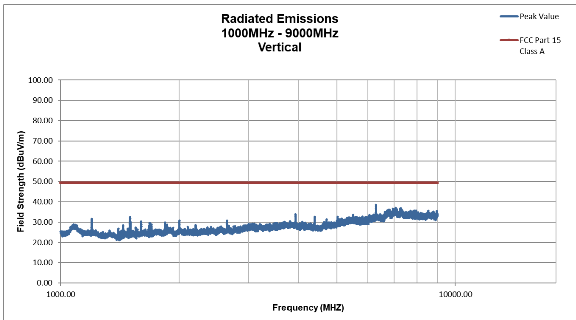
Figure 81. 775 MHz Vertical, Above 1000 MHz
