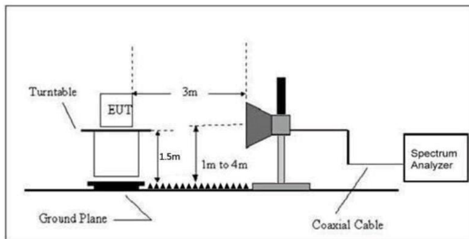
Figure 73. Radiated Spurious Emissions configurations
