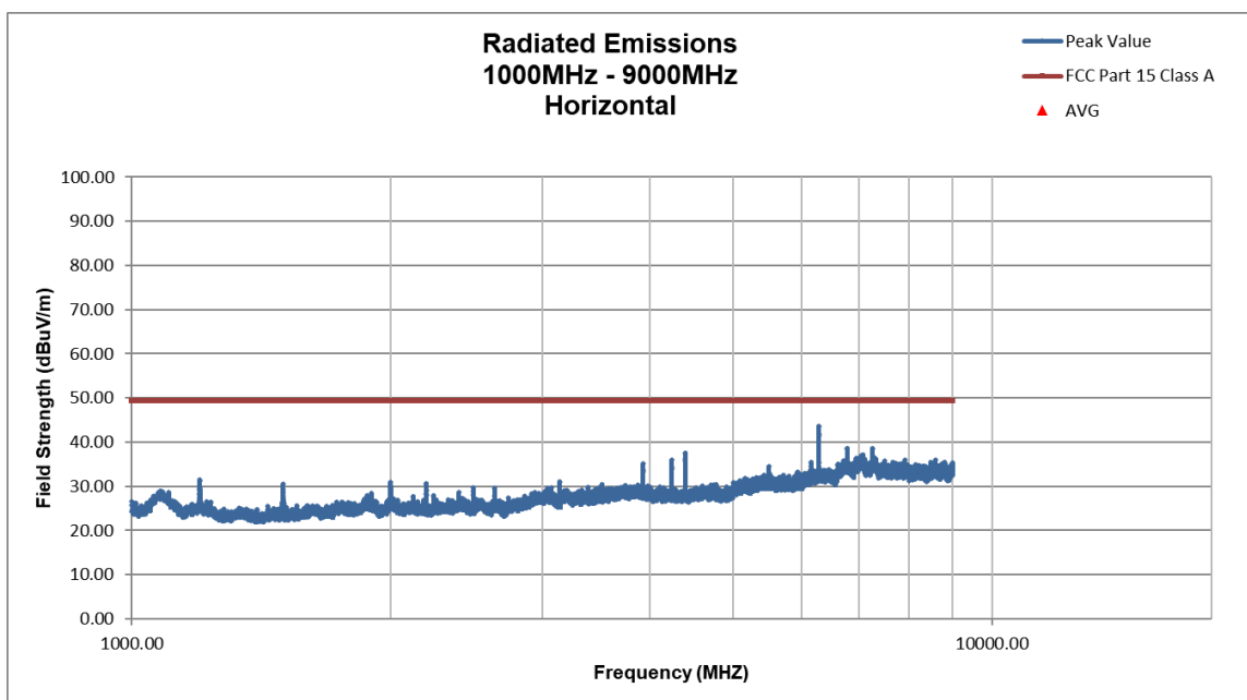
Figure 96. 799 MHz Horizontal, Above 1000 MHz
