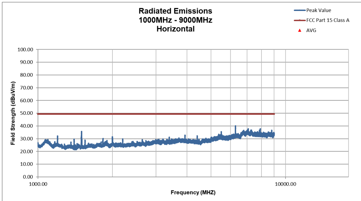
Figure 80. 775 MHz Horizontal, Above 1000 MHz
