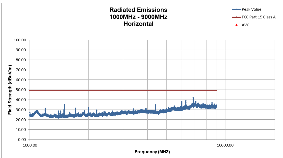
Figure 88. 856 MHz Horizontal, Above 1000 MHz
