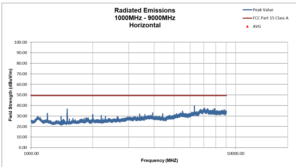
Figure 76. 769 MHz Horizontal, Above 1000 MHz
