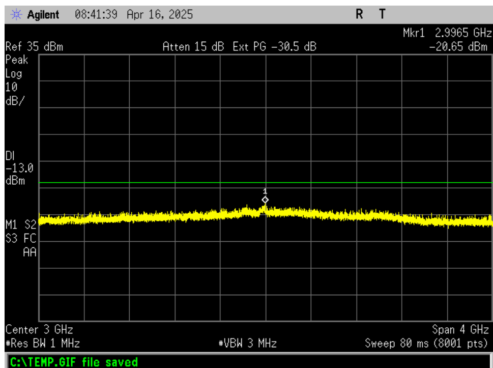
Figure 130. 775 MHz, 1 - 5 GHz
