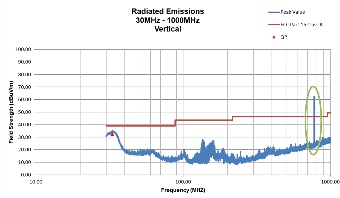
Figure 79. 775 MHz Vertical, 30 - 1000 MHz
