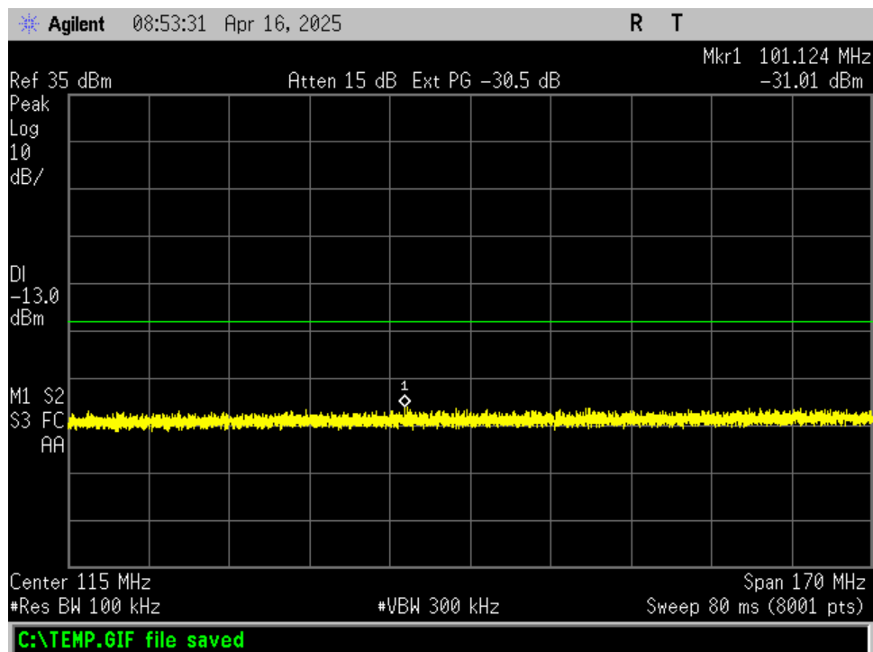
Figure 132. 851 MHz 30 - 200 MHz
