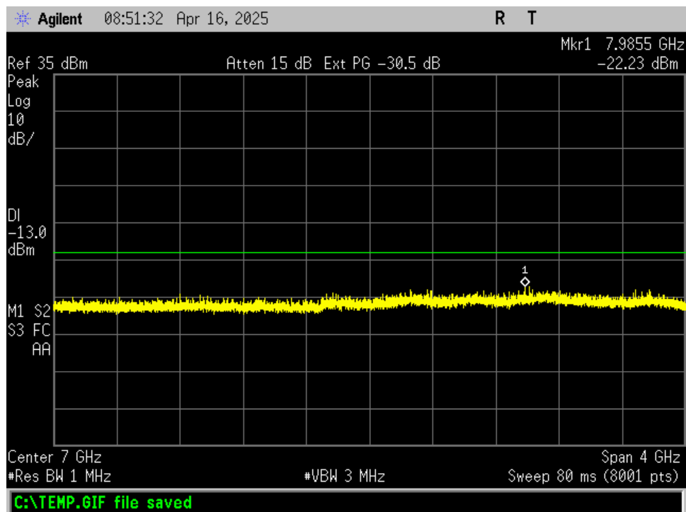
Figure 116. 808 MHz, 5 - 9 GHz
