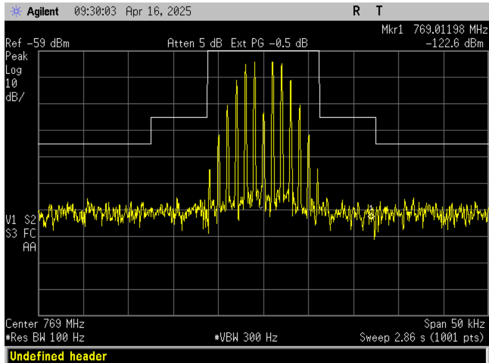
Figure 30. Input 769 MHz @ 12.5 kHz
