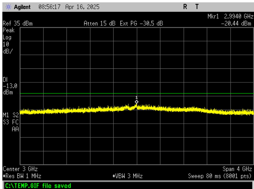
Figure 140. 856 MHz, 1 - 5 GHz
