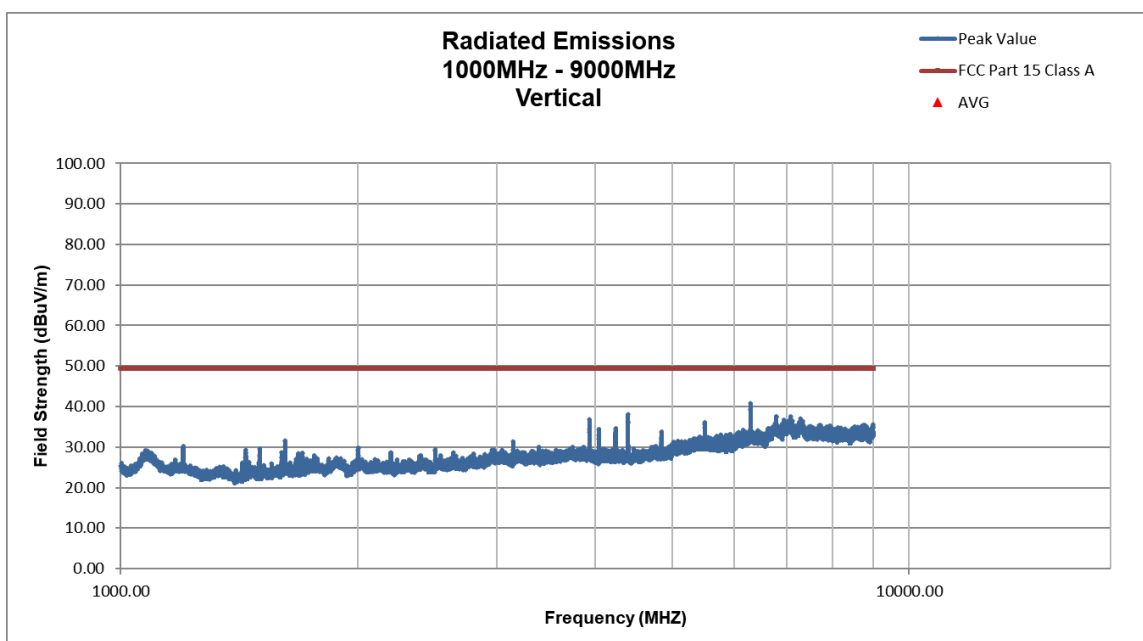
Figure 101. 808 MHz Vertical, Above 1000 MHz
