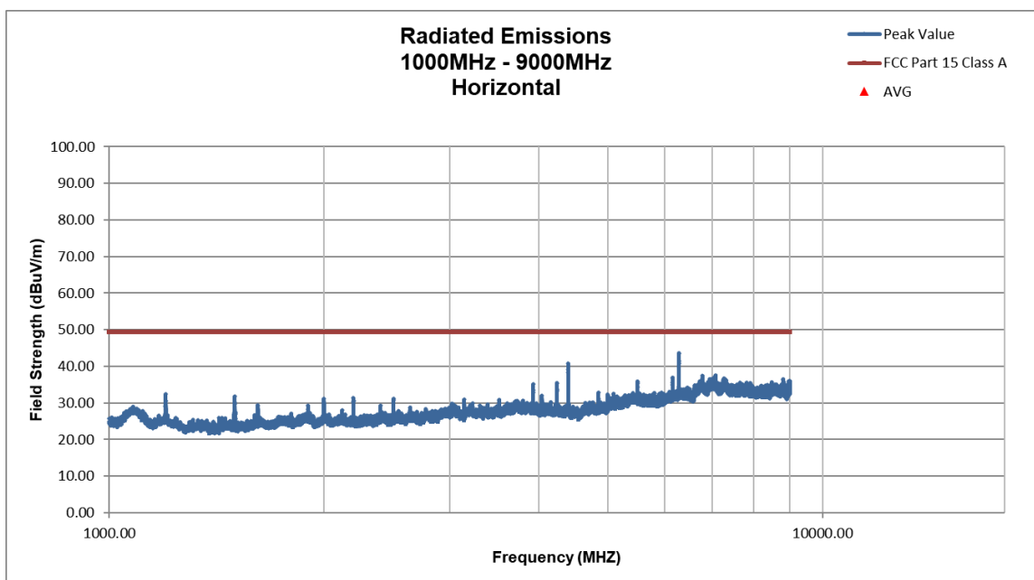
Figure 100. 808 MHz Horizontal, Above 1000 MHz
