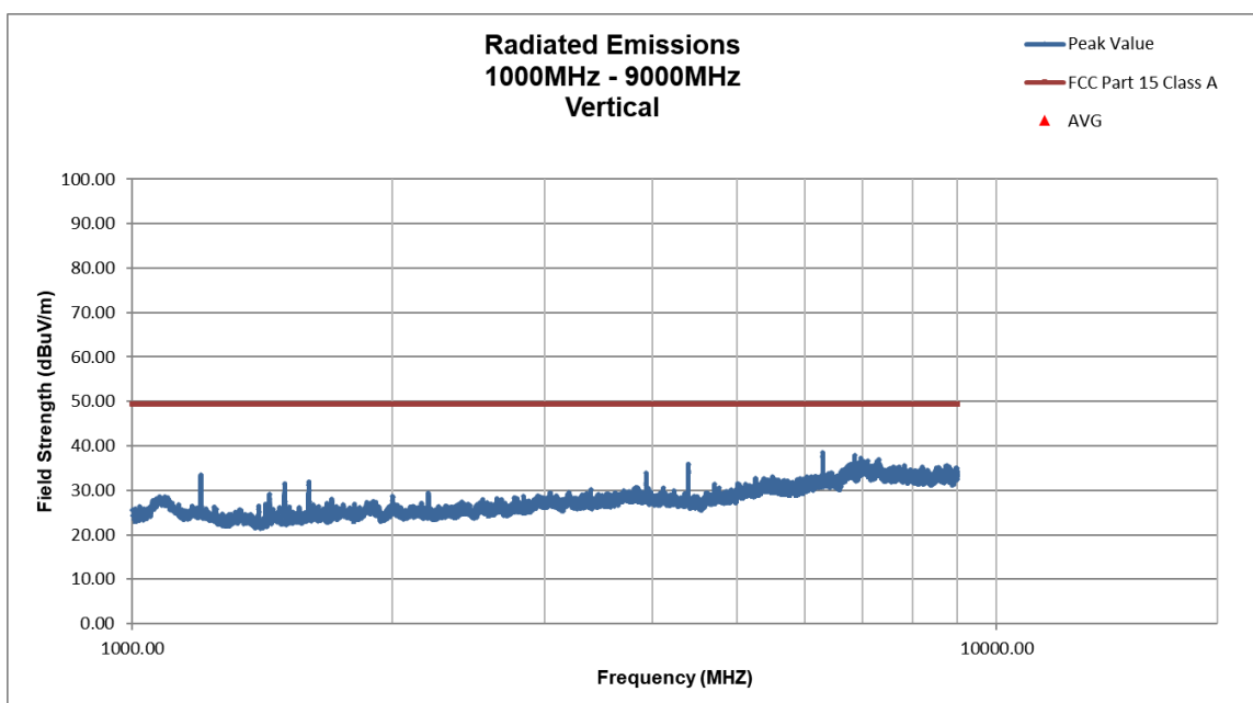
Figure 89. 856 MHz Vertical, Above 1000 MHz
