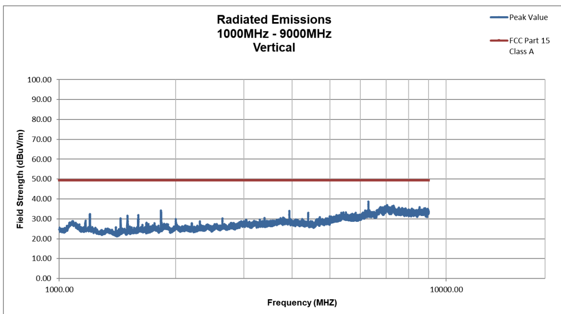
Figure 77. 769 MHz Vertical, Above 1000 MHz
