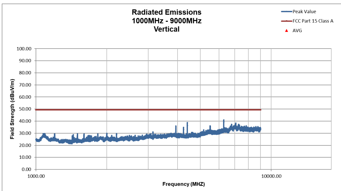
Figure 97. 799 MHz Vertical, Above 1000 MHz
