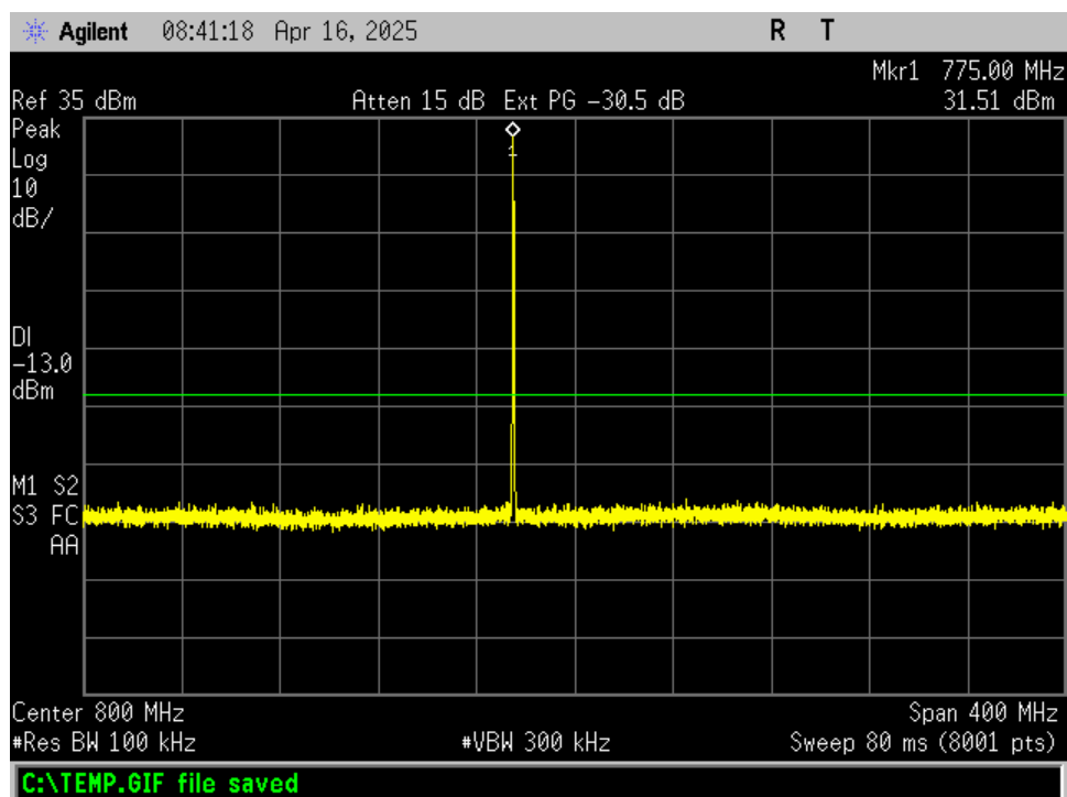
Figure 129. 775 MHz 600 - 1000 MHz
