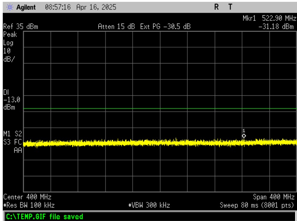
Figure 143. 861 MHz, 200 – 600 MHz
