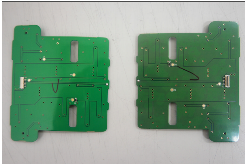
Bottom view of Sub PCB2 & 3
