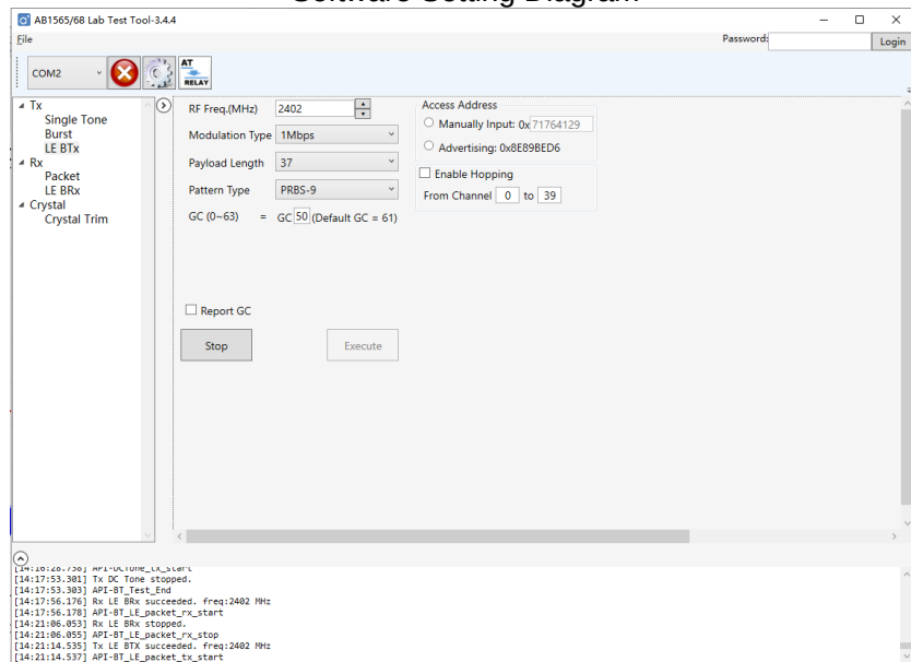
Software Setting Diagram
