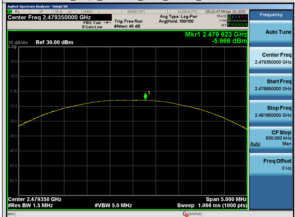
Test_Graph_SRD 2.4G_ANT1_2479.35_Peak Power
