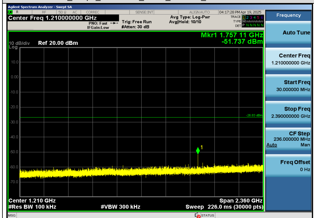
Test_Graph_SRD 2.4G_ANT0_2403.35_Lower Band Emissions
