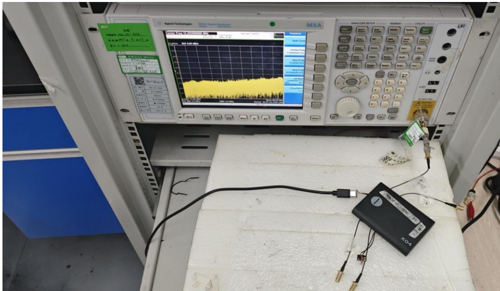
RF CONDUCTED TEST SETUP-Model 2# ANT 0
