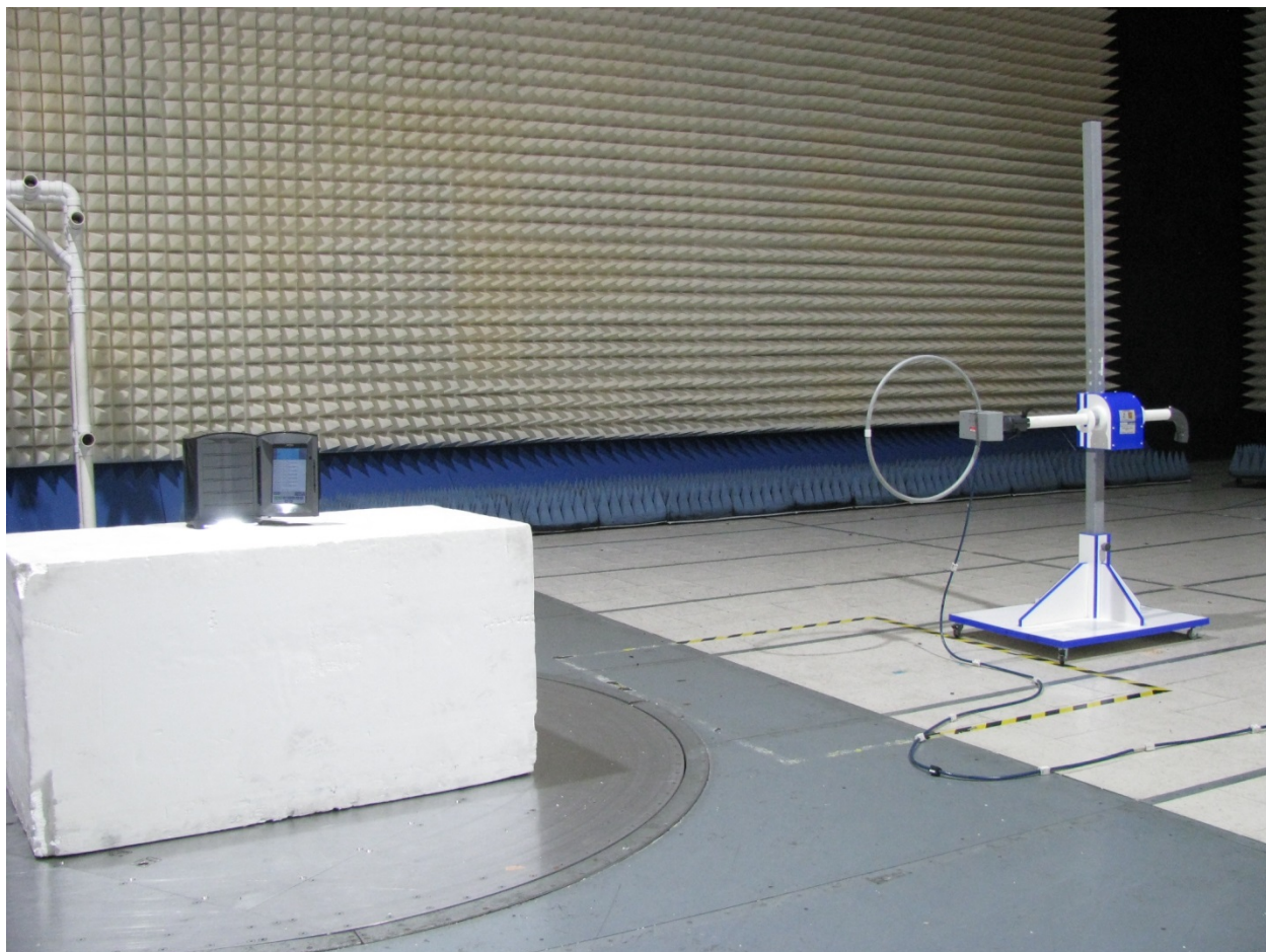
Radiated emissions, 10kHz – 30MHz
