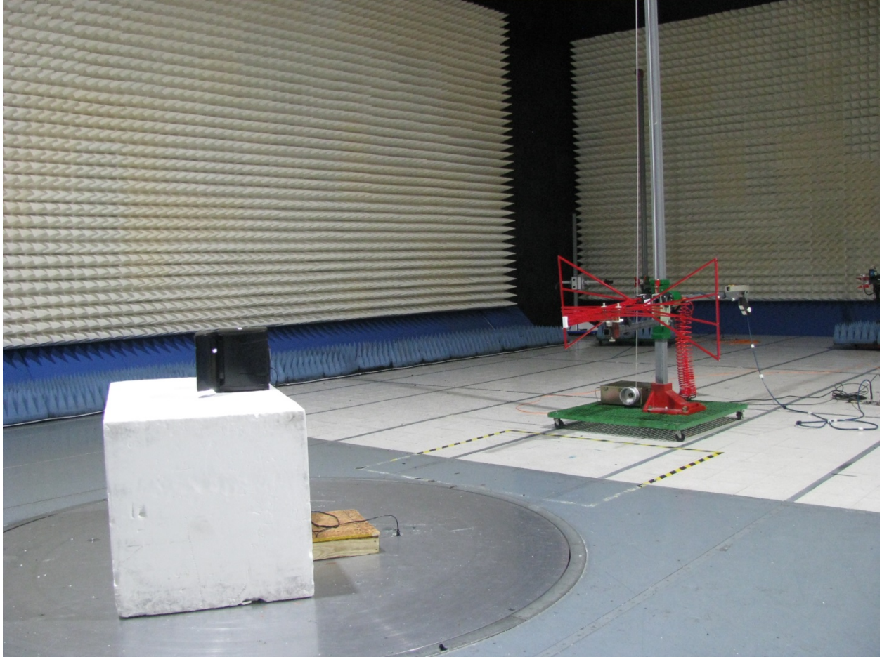
Radiated emissions, 80MHz – 1GHz
