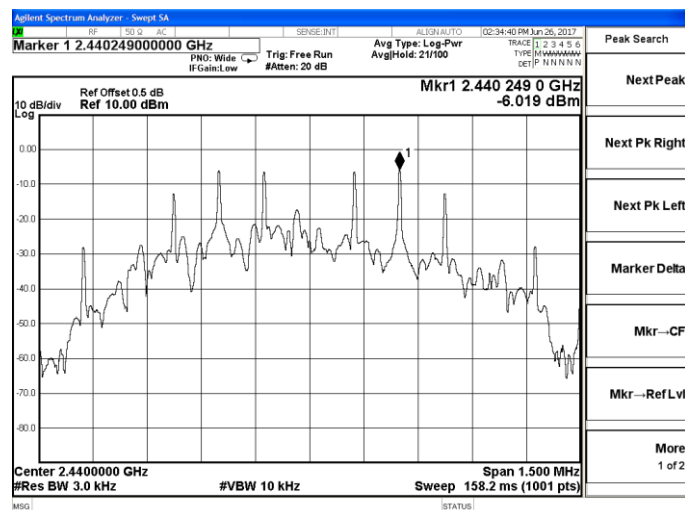
Channel 19 / 2440 MHz
