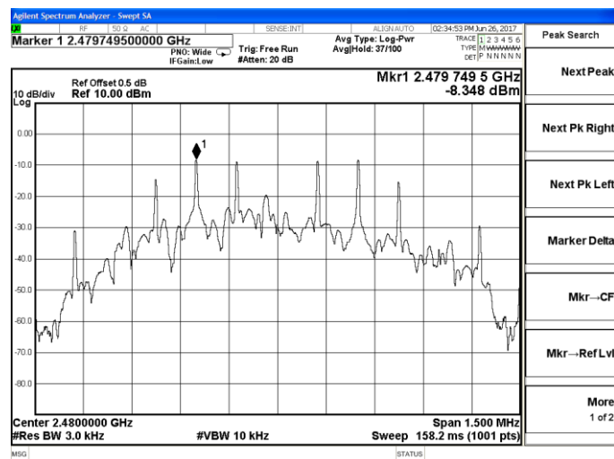
Channel 39 / 2480 MHz
