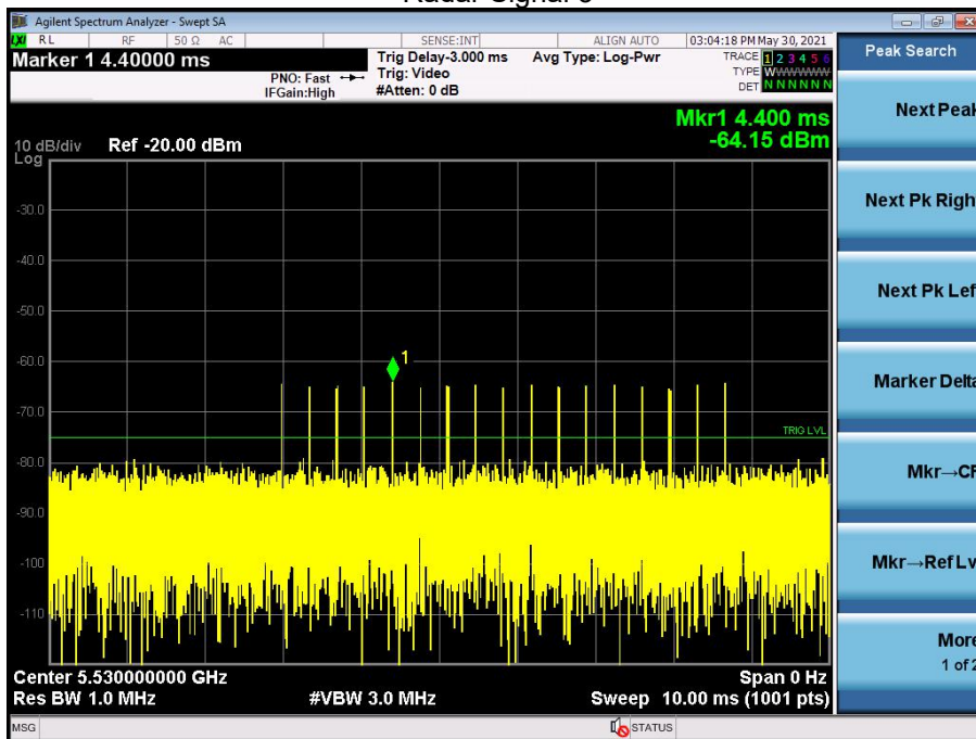
Radar Signal 3
