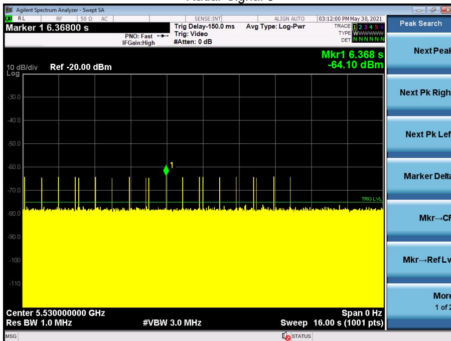
Radar Signal 5
