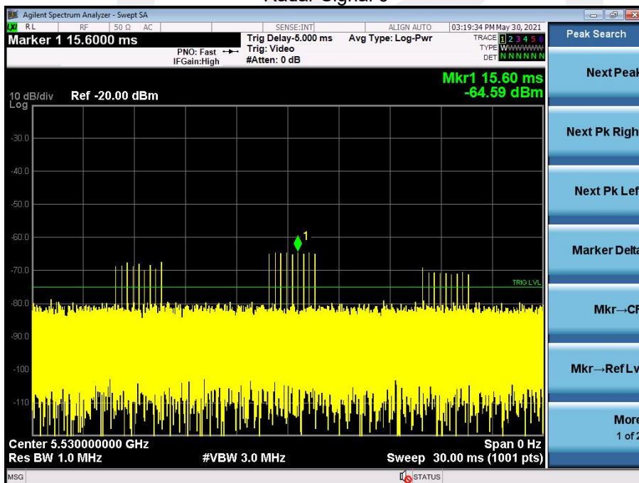
Radar Signal 6
