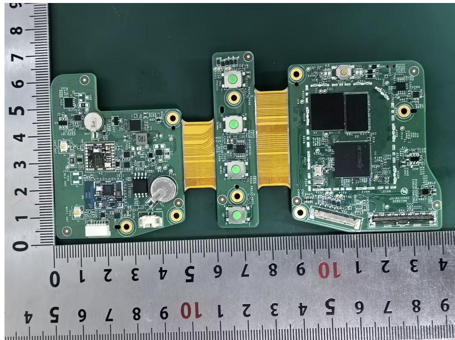
EUT View 14
