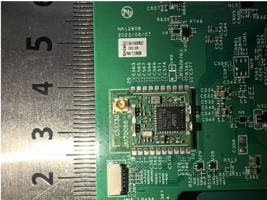
EUT View 16
