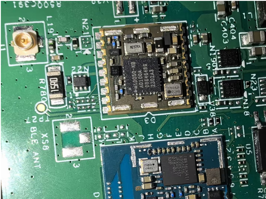
EUT View 15
