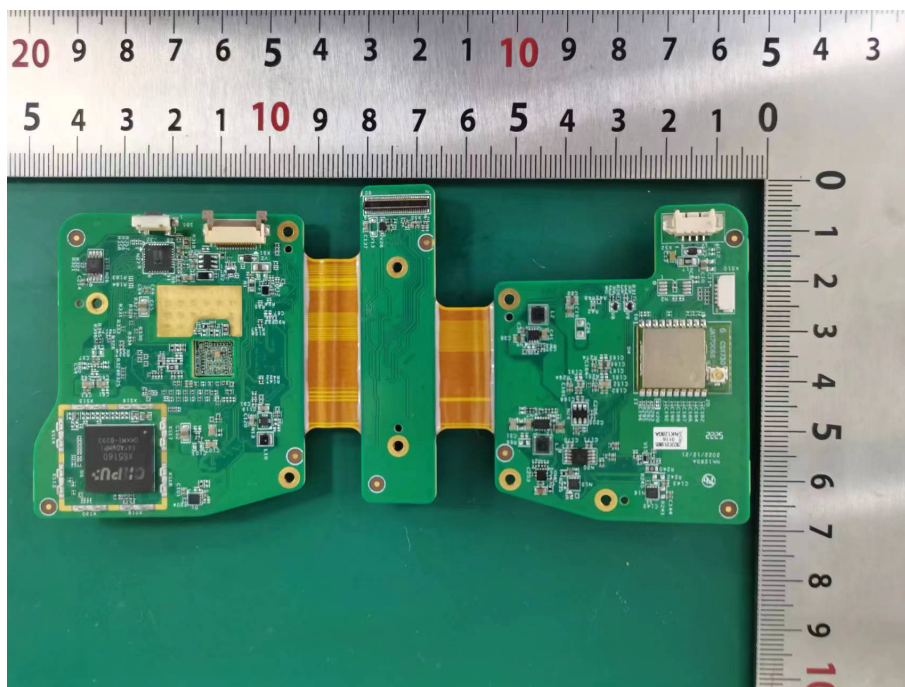
EUT View 12
