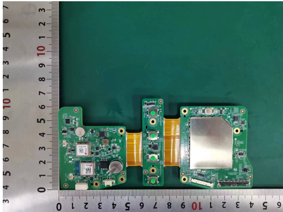
EUT View 13
