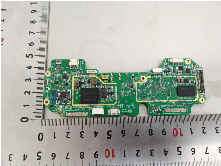
EUT View 4
