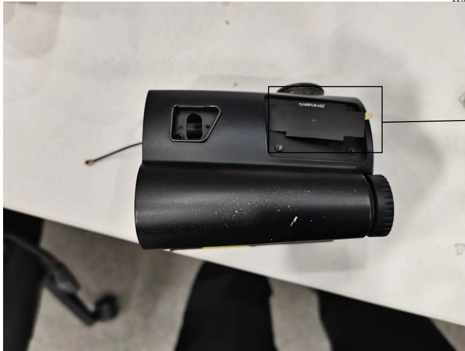
FPC Antenna
