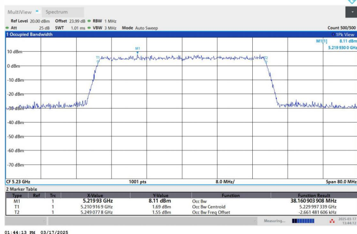
11AX40SISO-Ant1-5230
