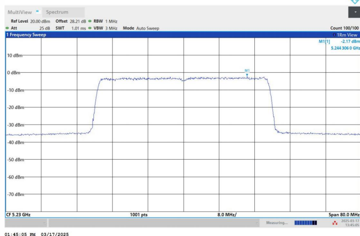
11AX40SISO-Ant1-5230-PASS
