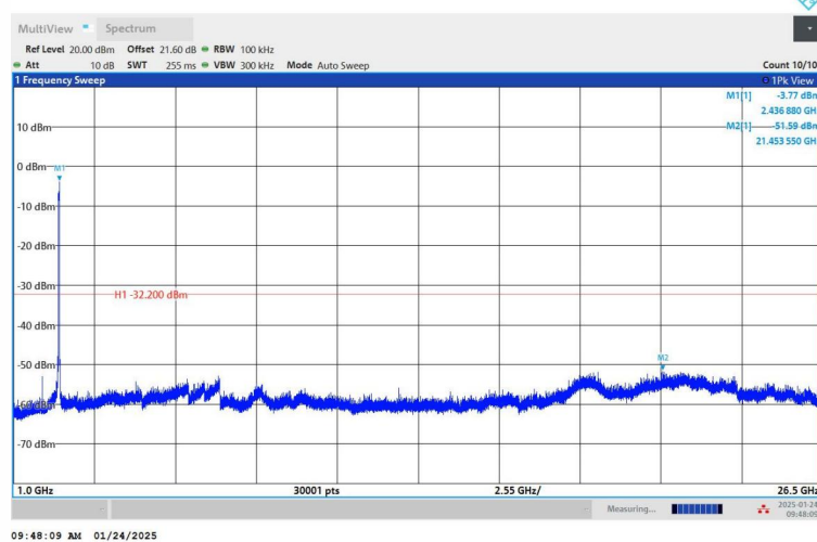
11N40SISO_Ant1_2437_0~Reference
