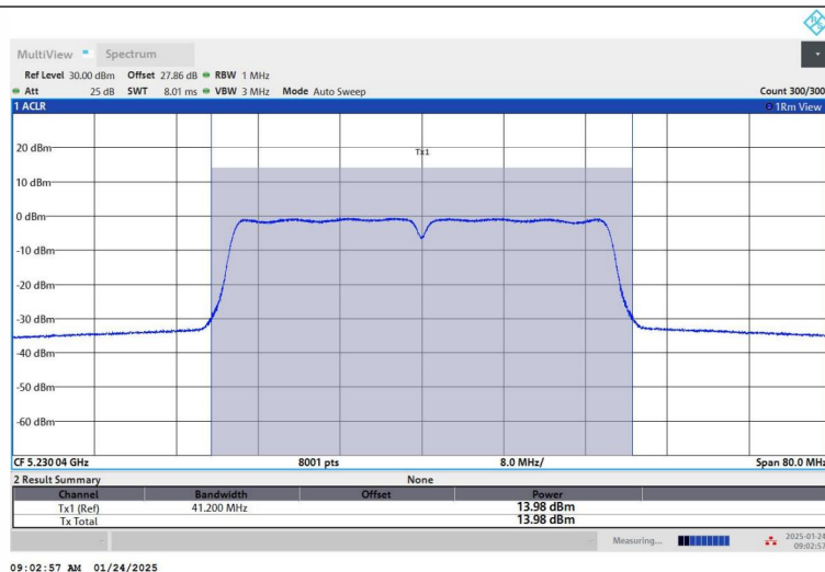
11AX20SISO_Ant1_5180
