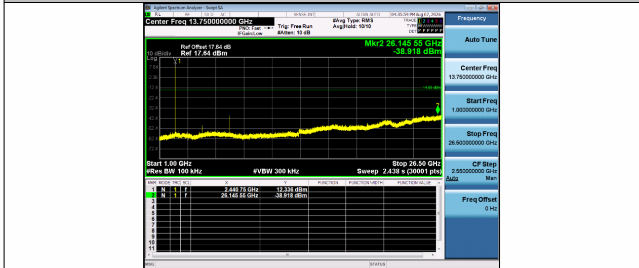
DH5-Ant1-2441-1000~26500-PASS
