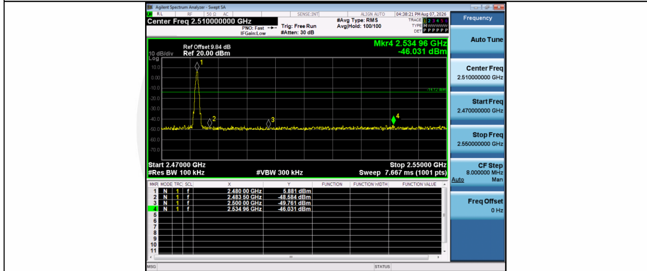
DH5-Ant1-2480-PASS
