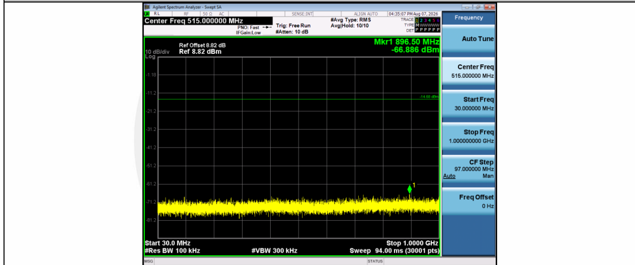
DH5-Ant1-2441-30~1000-PASS
