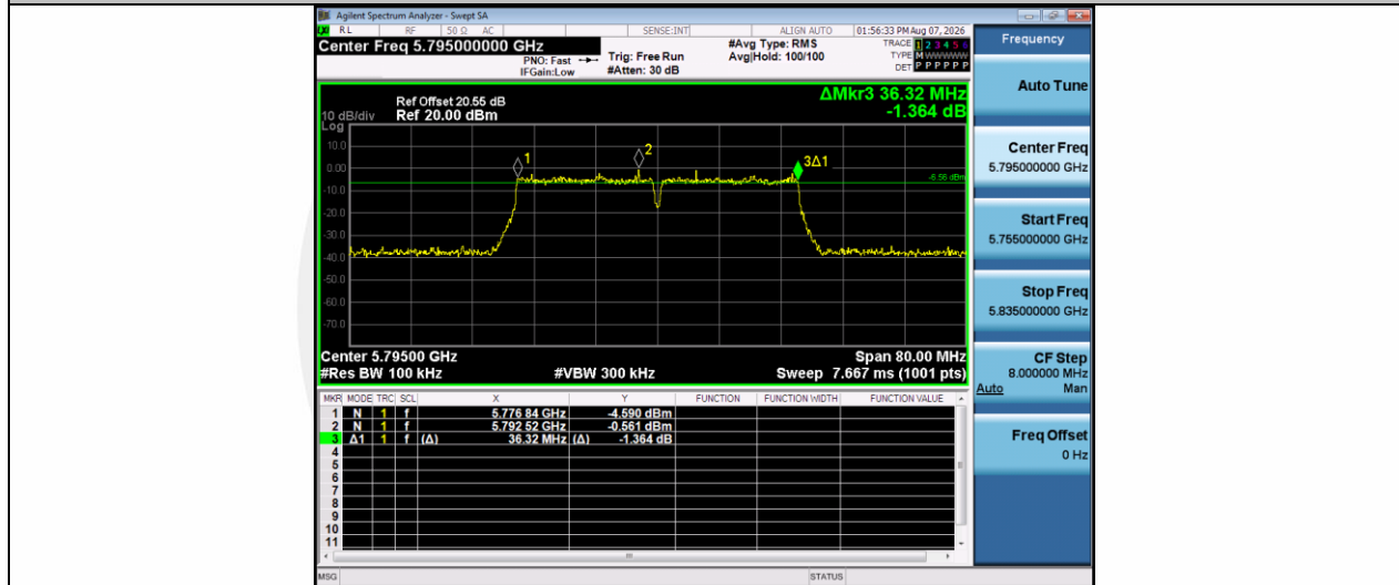
11N40SISO-Ant1-5795-PASS
