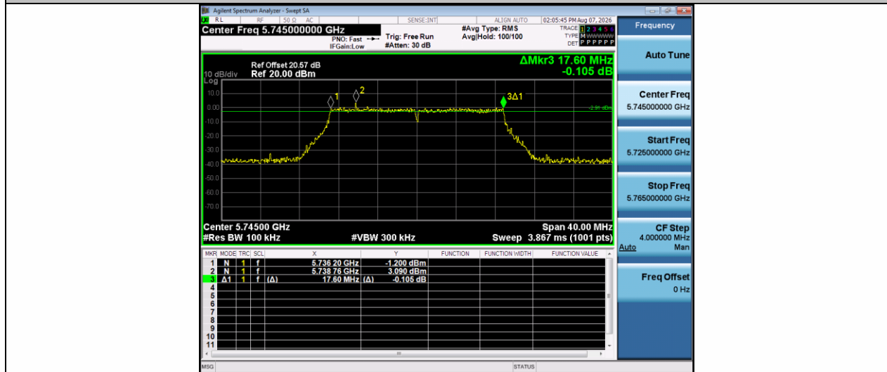
11AC20SISO-Ant1-5745-PASS
