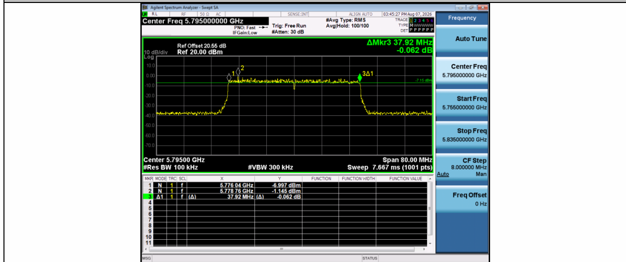
11AX40SISO-Ant1-5795-PASS
