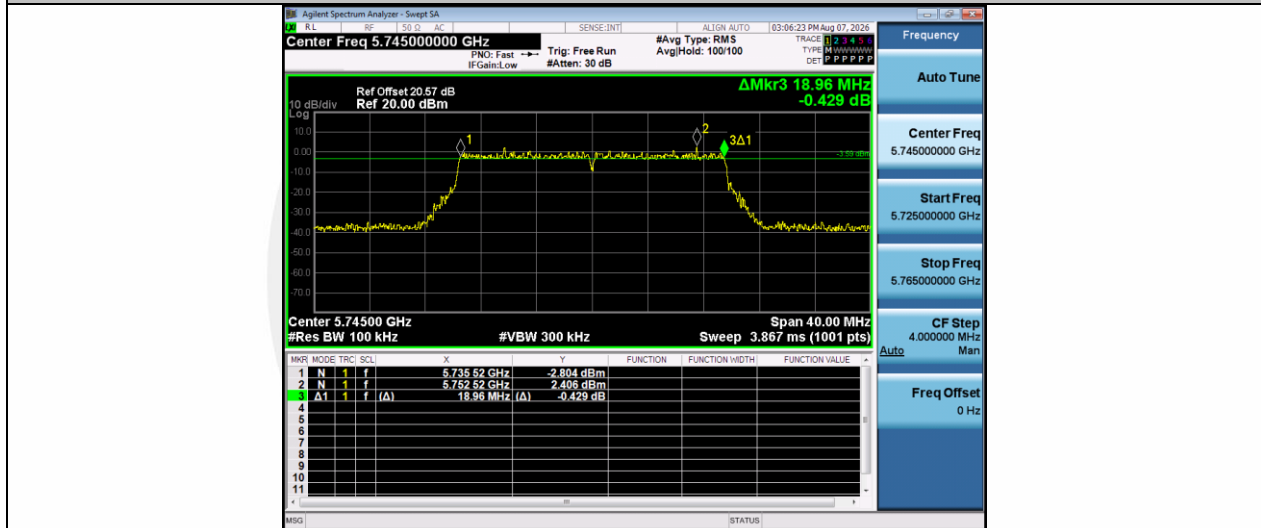
11AX20SISO-Ant1-5745-PASS
