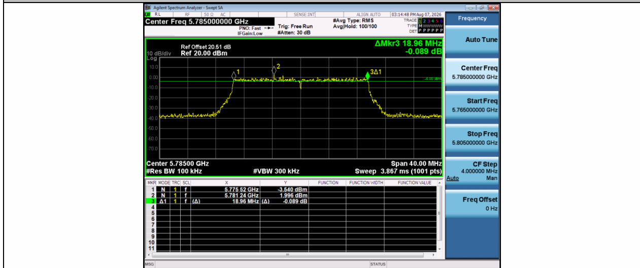
11AX20SISO-Ant1-5785-PASS
