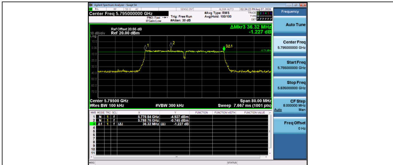
11AC40SISO-Ant1-5795-PASS
