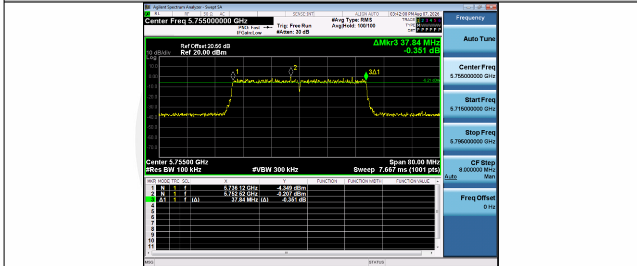
11AX40SISO-Ant1-5755-PASS
