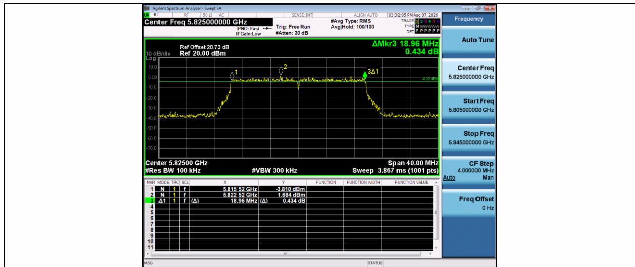
11AX20SISO-Ant1-5825-PASS
