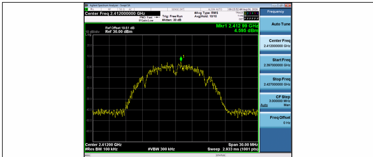
11B-Ant1-2412-0~Reference-PASS
