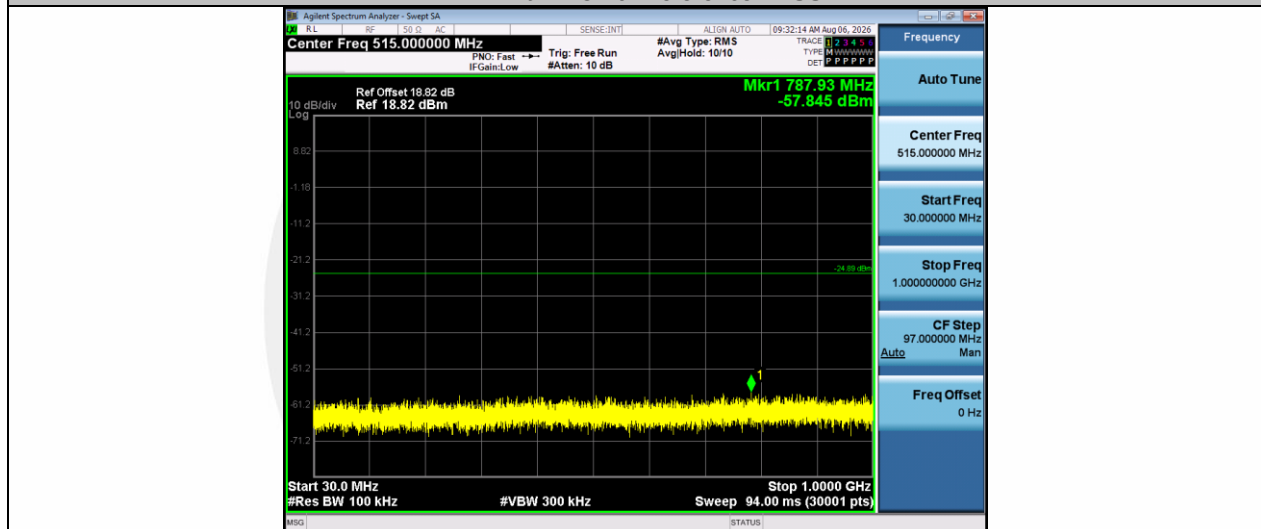
11B-Ant1-2437-30~1000-PASS
