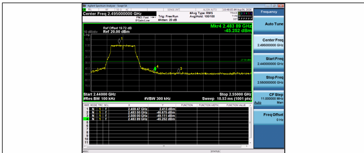
11G-Ant1-2462-PASS
