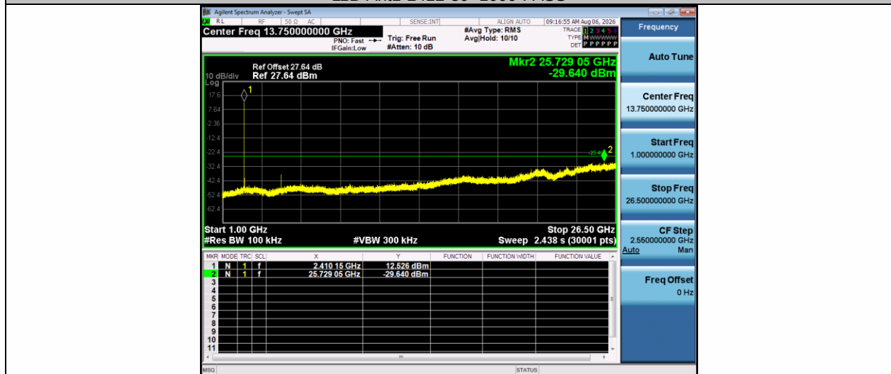
11B-Ant1-2412-1000~26500-PASS
