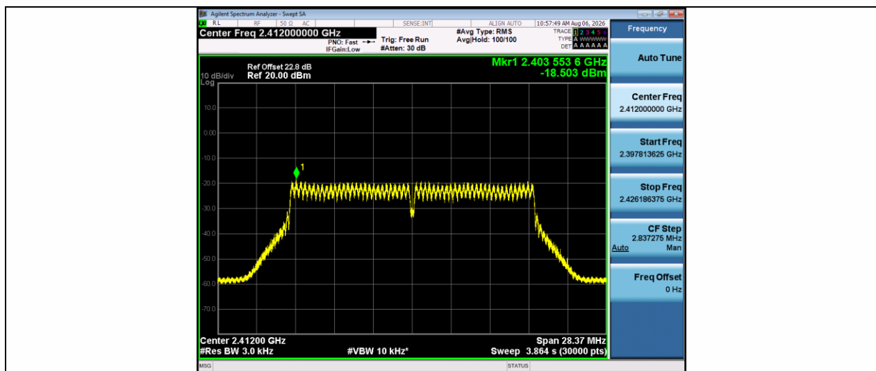
11N20SISO-Ant1-2412-PASS
