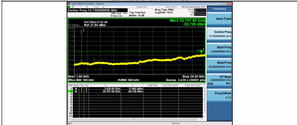
11B-Ant1-2437-1000~26500-PASS
