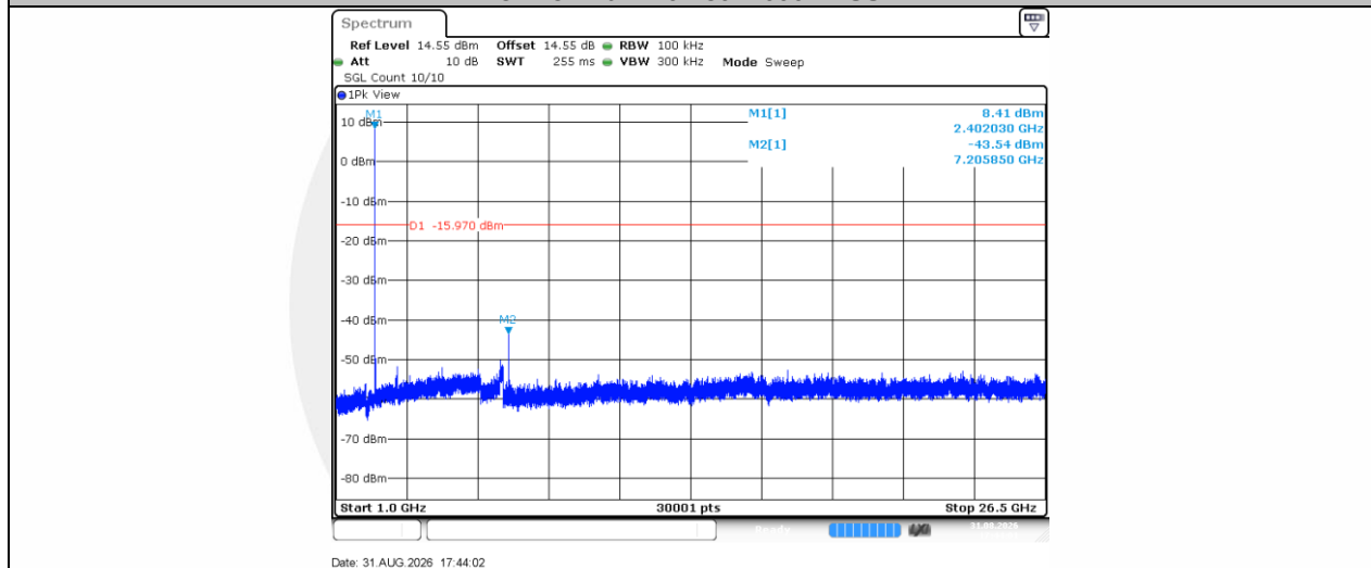
3DH5-Ant1-2402-1000~26500-PASS
