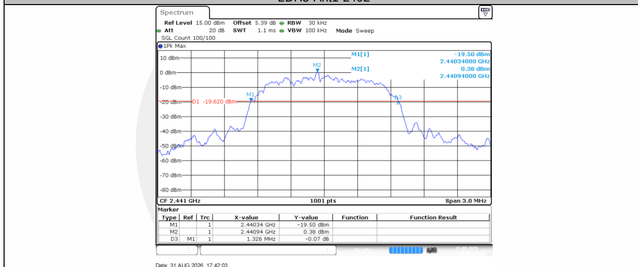
2DH5-Ant1-2441
