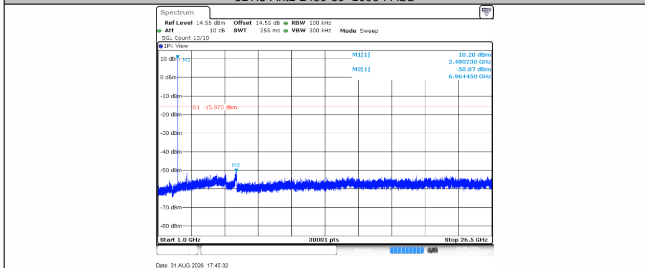
3DH5-Ant1-2480-1000~26500-PASS
