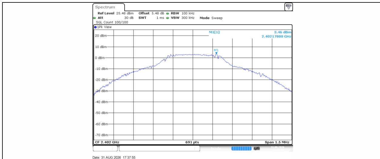
DH5-Ant1-2402-PASS
