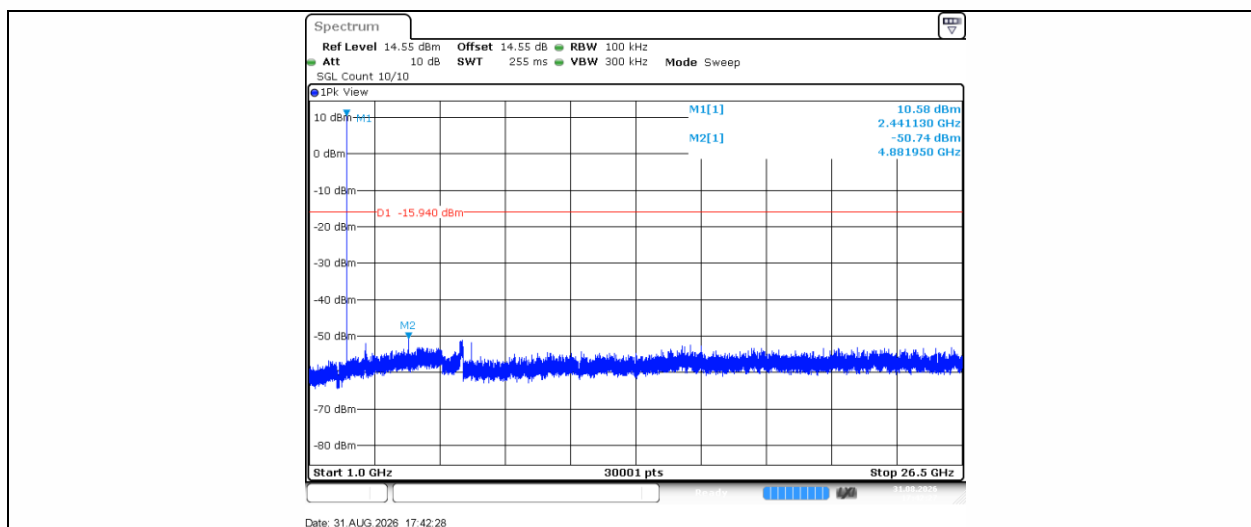
2DH5-Ant1-2441-1000~26500-PASS
