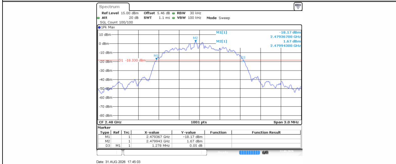
3DH5-Ant1-2480
