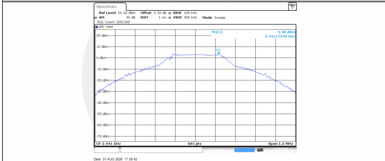
DH5-Ant1-2441-PASS
