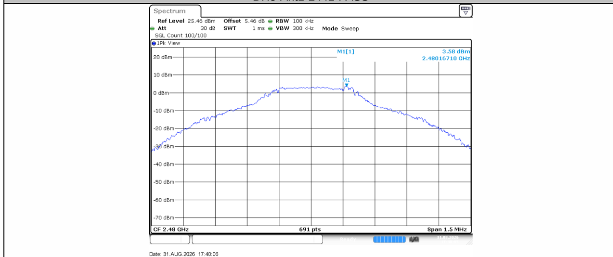
DH5-Ant1-2480-PASS
