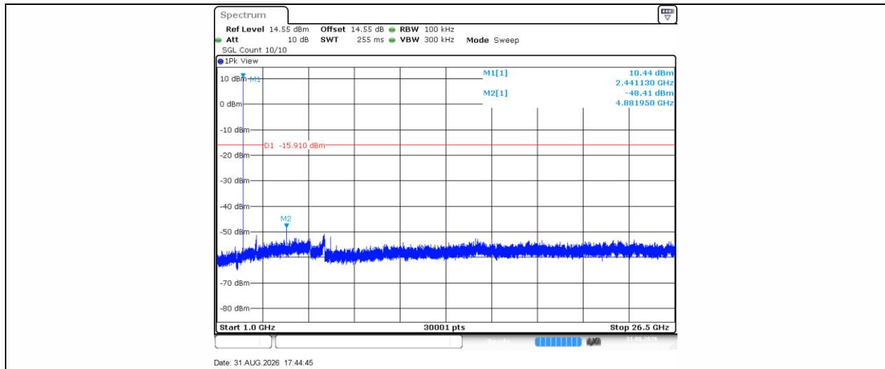
3DH5-Ant1-2441-1000~26500-PASS
