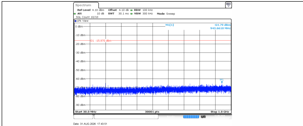
3DH5-Ant1-2402-30~1000-PASS
