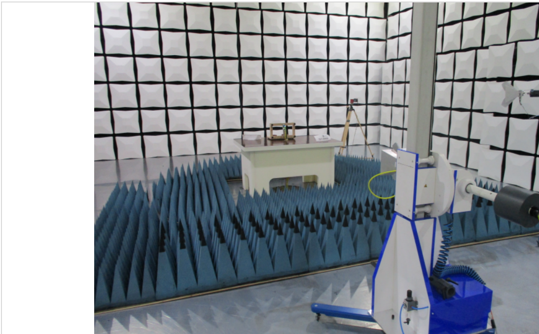
Photograph 2: Radiated emission measurements test set-up for measurement of frequency above 1 GHz Final measurement in 3 m test distance
