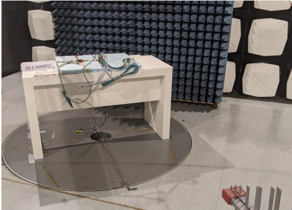
Photograph 1: EUT Test Setup in the semi anechoic chamber, Radiated interference field strength
