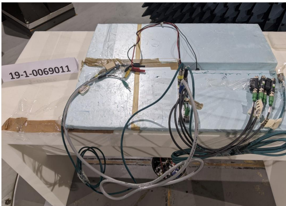
Photograph 2: EUT Test Setup in the semi anechoic chamber, Radiated interference field strength
