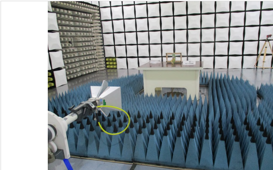
Photograph 2: Radiated emission measurements test set-up for measurement of frequency above 1 GHz Final measurement in 3 m test distance
