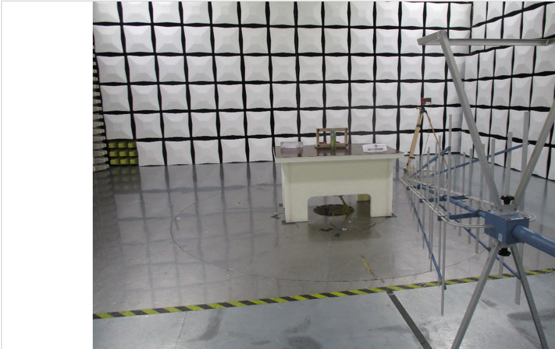
Photograph 1: Radiated emission measurements test set-up for measurement of frequency up to 1000 MHz Preliminary measurement in 3 m test distance
