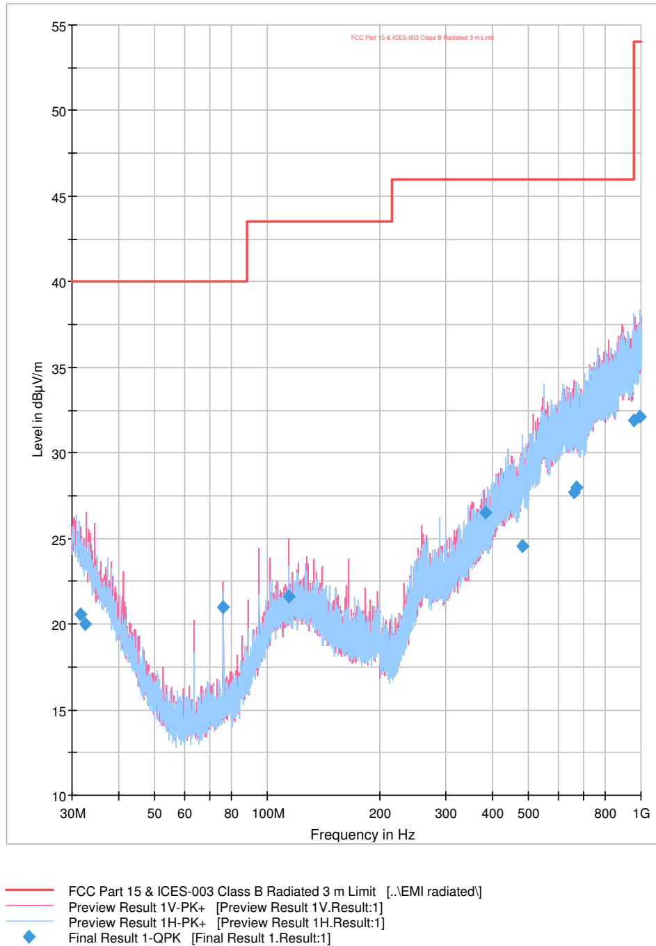
Figure 2.7.10-1 – Receive Mode Radiated Emissions Plot
