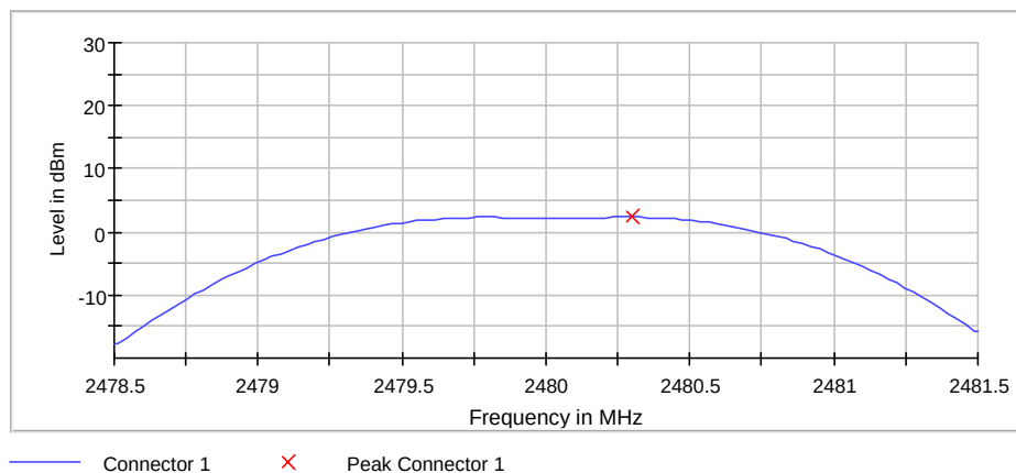
Figure 7.4.2-1: Sample Plot
