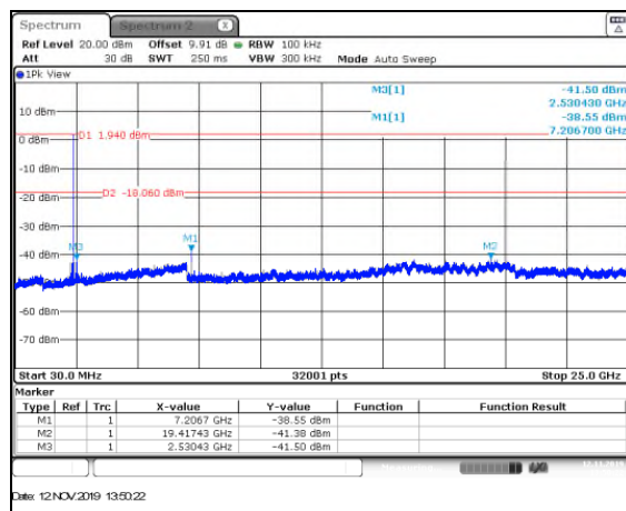
Figure 7.5.1.2-1: LCH – 30MHz–25GHz
