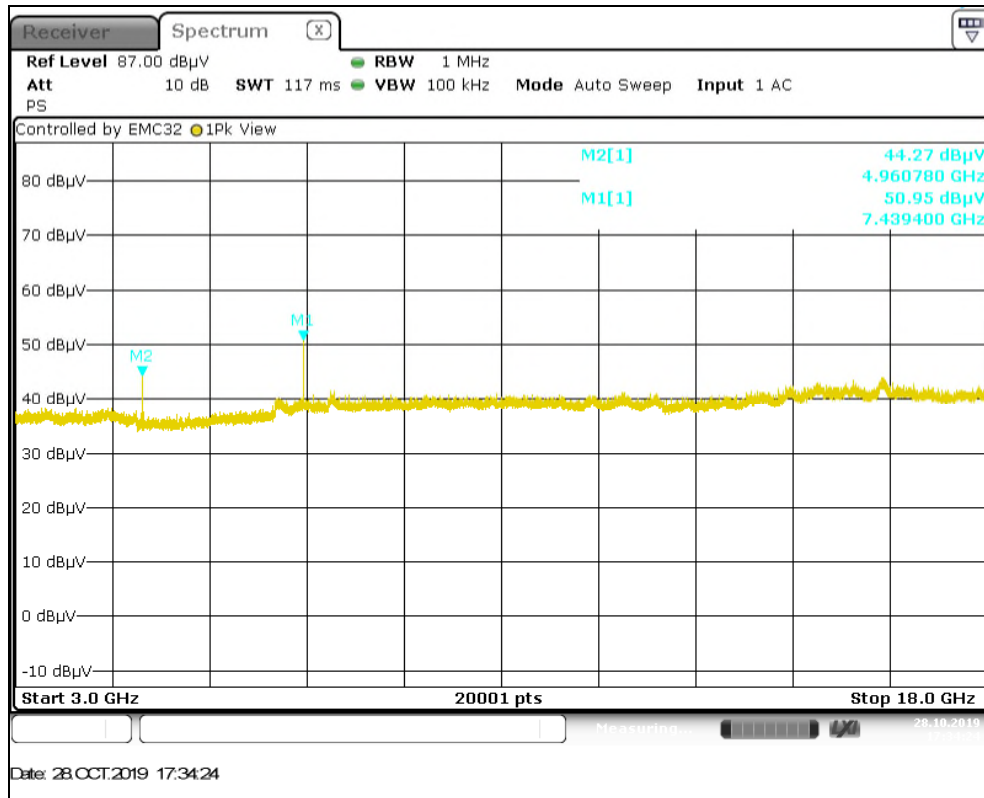
Figure A-5: 3GHz-18GHz
