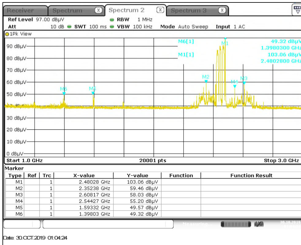
Figure A-4: 1GHz-3GHz
