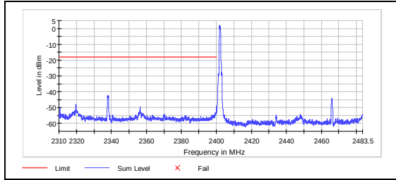
Figure 7.5.1.2-4: Lower Band-edge
