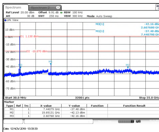
Figure 7.5.1.2-3: HCH – 30MHz–25GHz
