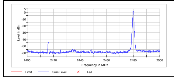
Figure 7.5.1.2-5: Upper Band-edge
