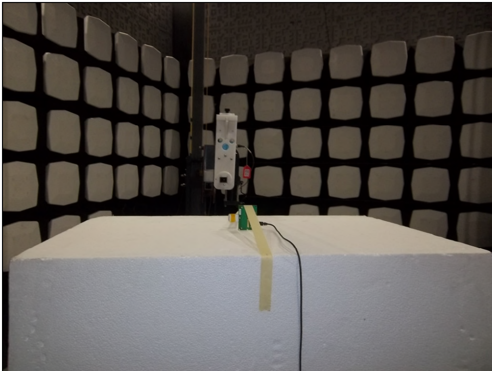
Figure 13: Equipment Under Test – Radiated Emissions >18GHz
