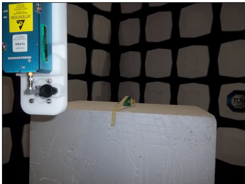
Figure 12: Equipment Under Test – Radiated Emissions >18GHz
