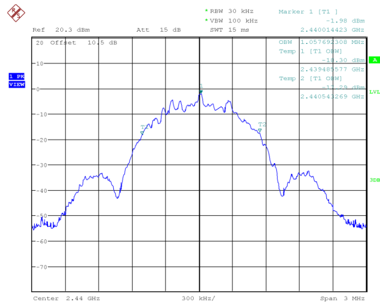
Figure 14: 2440MHz, 1Mbps, 99% Bandwidth
