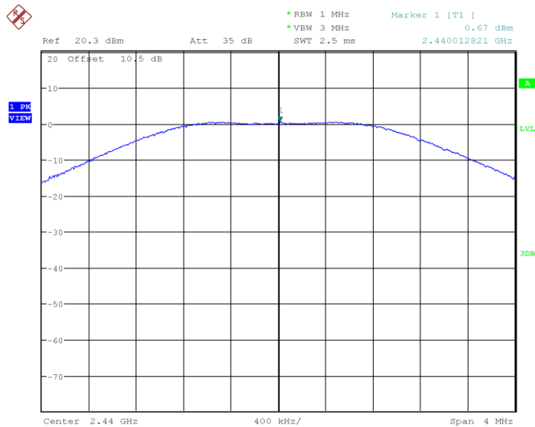
Figure 5: Maximum Conducted Power, 2440MHz, 2Mbps
