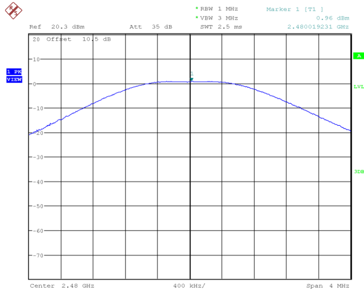
Figure 3: Maximum Conducted Power, 2480MHz, 1Mbps
