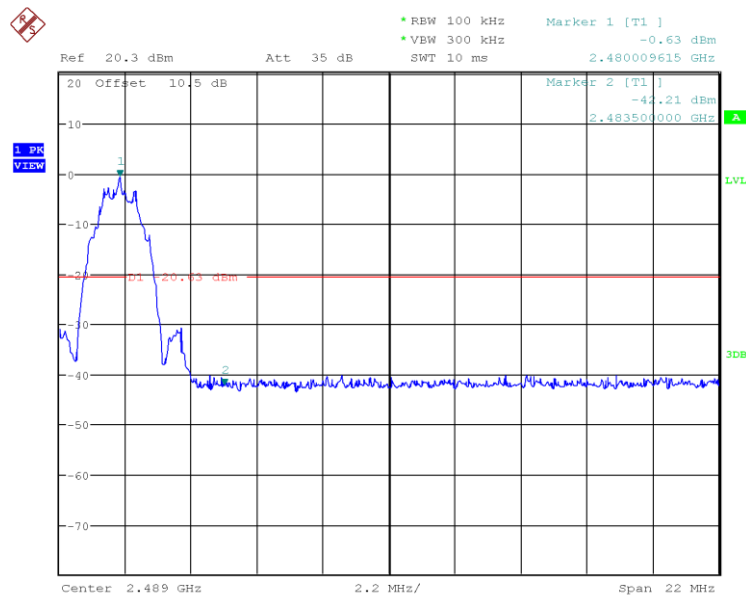
Figure 28: 2480MHz, 2Mbps Upper Band Edge
