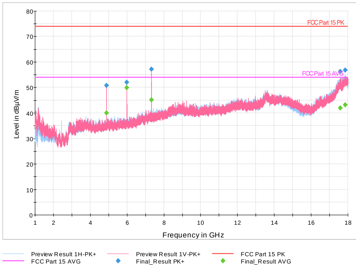
Figure 43: Radiated Spurious Emissions 1GHz - 18GHz, 2440MHz, 1Mbps
