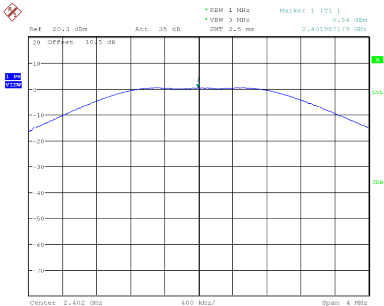
Figure 4: Maximum Conducted Power, 2402 MHz, 2Mbps
