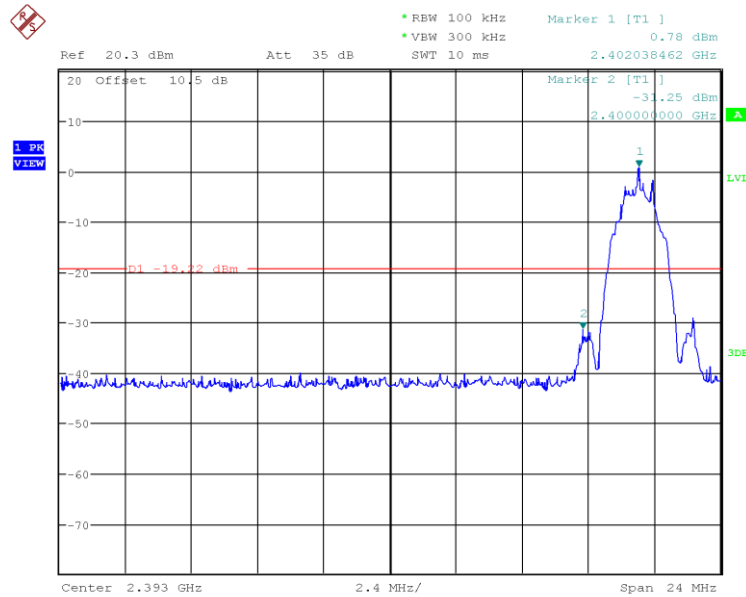
Figure 27: 2402MHz, 2Mbps, Lower Band Edge
