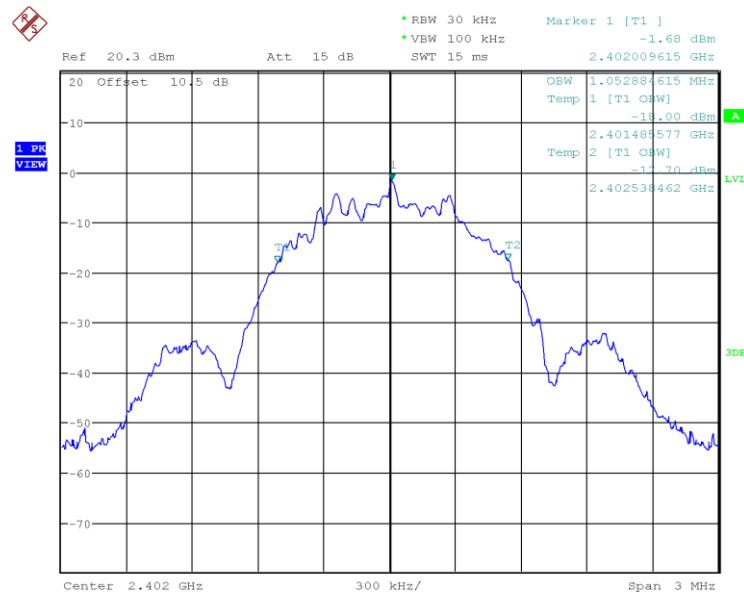
Figure 13: 2402MHz, 1Mbps, 99% Bandwidth
