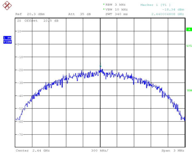
Figure 23: 2440 MHz, 2Mbps, PSD
