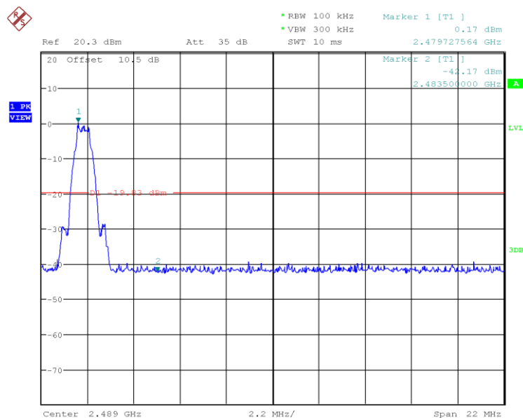
Figure 26: 2480MHz, 1Mbps Upper Band Edge
