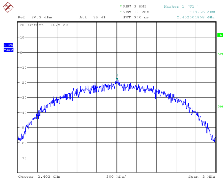
Figure 22: 2402 MHz, 2Mbps, PSD
