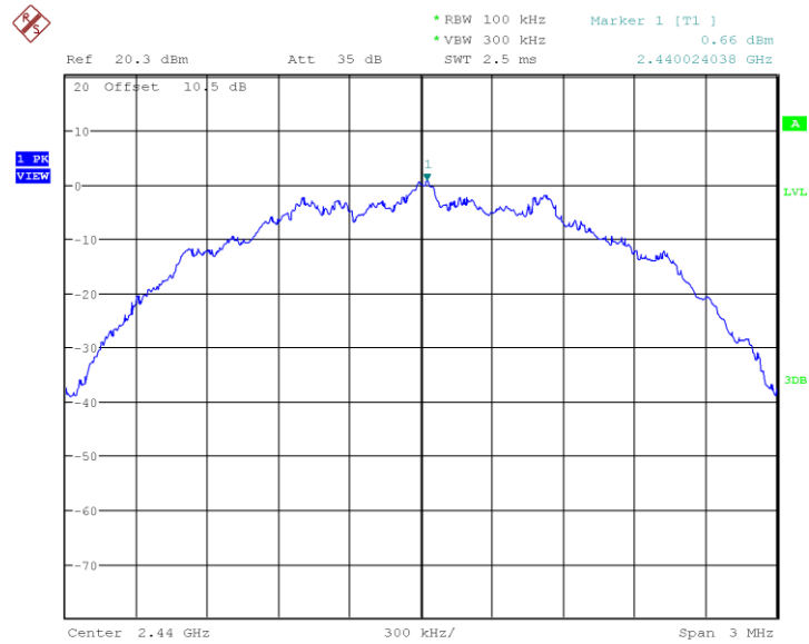
Figure 33: 2Mbps Ref Measurement
