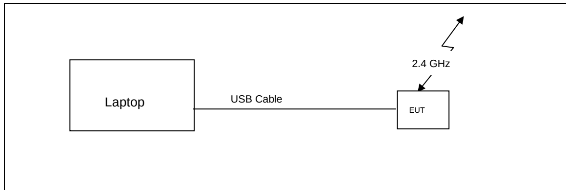
Figure 50: Block Diagram of EUT Setup - Radiated
