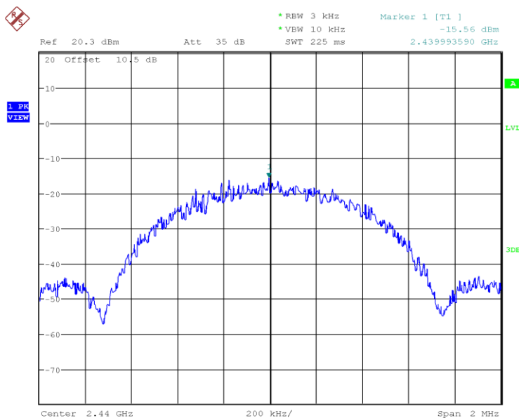
Figure 20: 2440 MHz, 1Mbps, PSD
