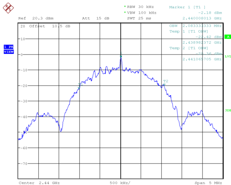
Figure 17: 2440MHz, 2Mbps, 99% Bandwidth
