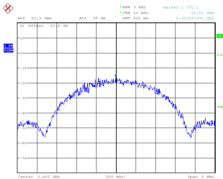
Figure 19: 2402 MHz, 1Mbps, PSD
