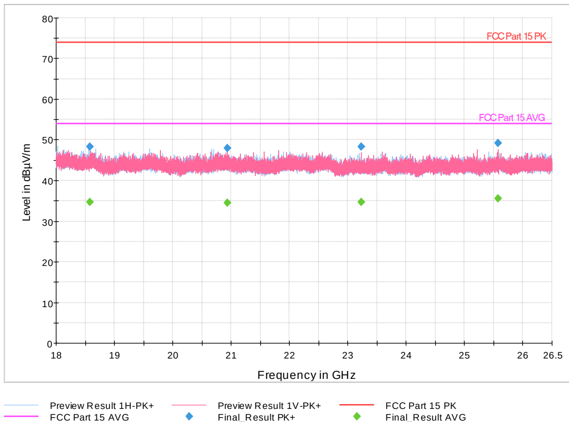
Figure 47: Radiated Spurious Emissions 18GHz - 26GHz, 2480MHz, 1Mbps
