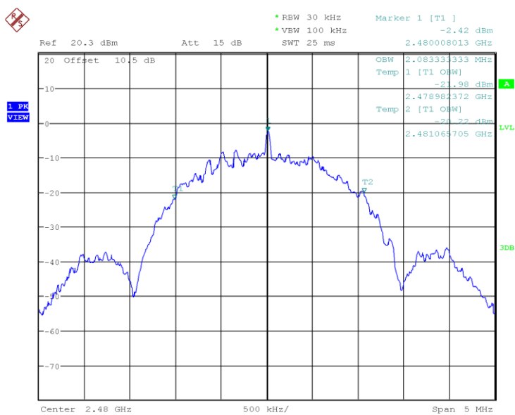
Figure 18: 2480MHz, 2Mbps, 99% Bandwidth
