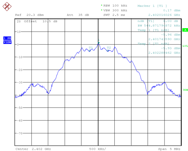
Figure 10: 2402MHz, 2Mbps, 6dB Bandwidth
