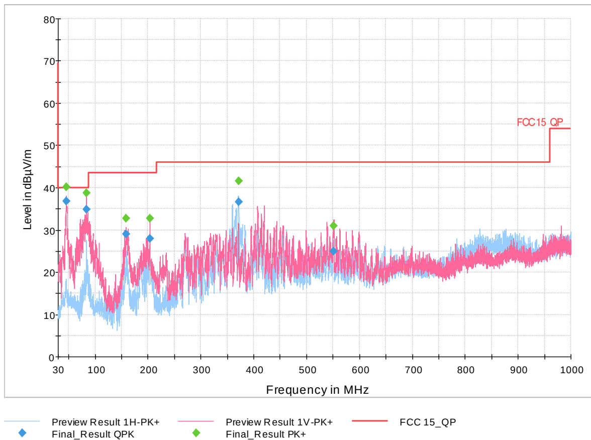
Figure 41: Radiated Spurious Emissions 30MHz – 1GHz, 2480MHz, 1Mbps
