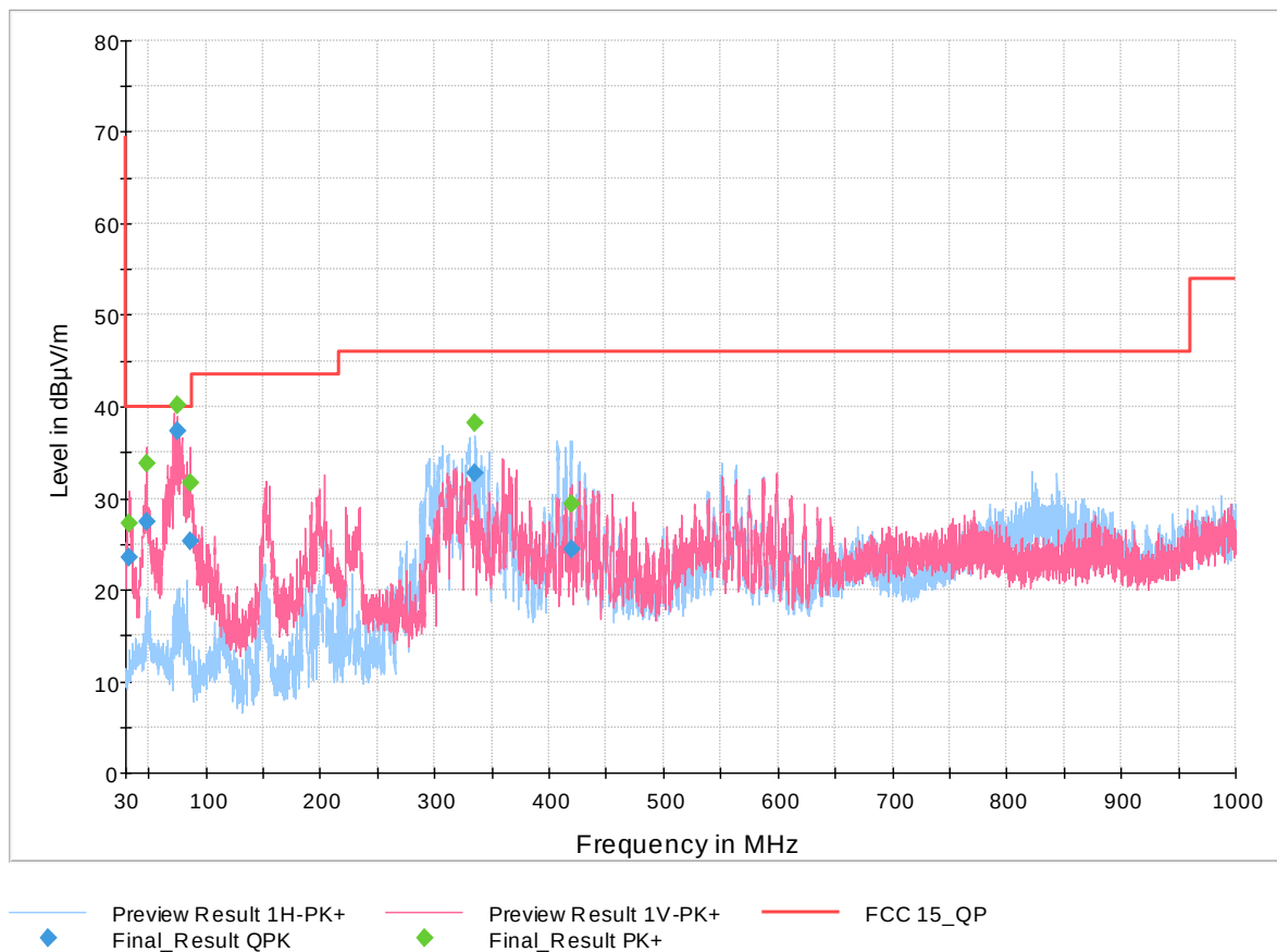
Figure 40: Radiated Spurious Emissions 30MHz – 1GHz, 2440MHz, 1Mbps
