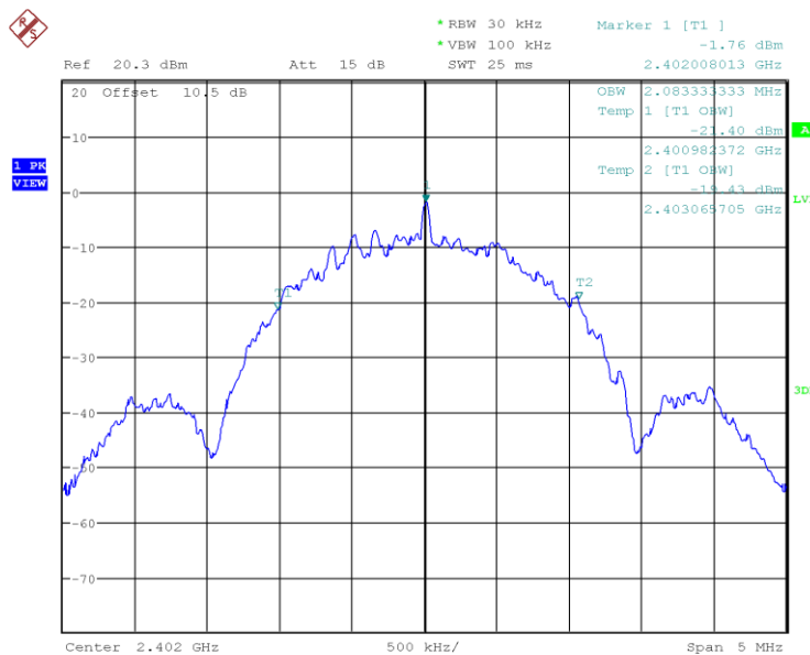
Figure 16: 2402MHz, 2Mbps, 99% Bandwidth
