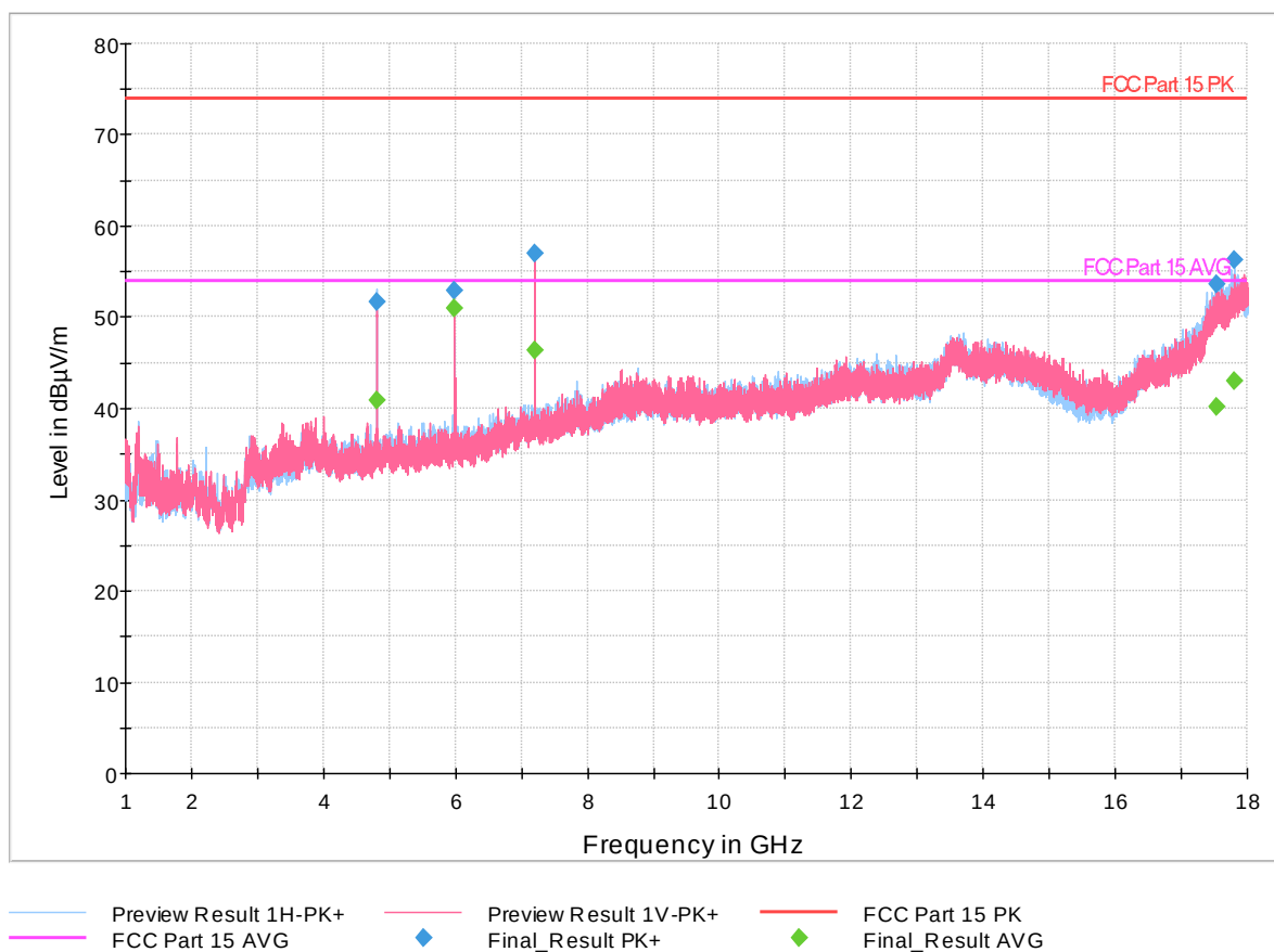
Figure 42: Radiated Spurious Emissions 1GHz - 18GHz, 2402MHz, 1Mbps
