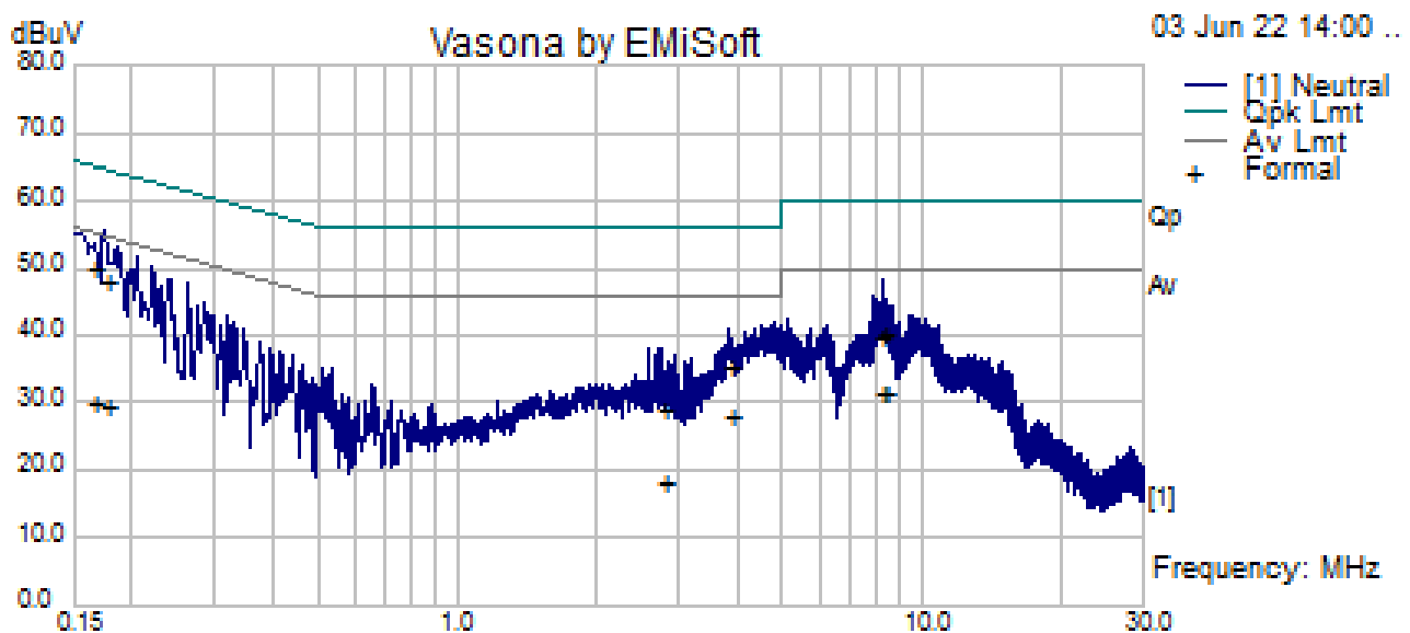
Figure 49: AC Conducted Emissions 150 kHz to 30 MHz – Neutral Line
