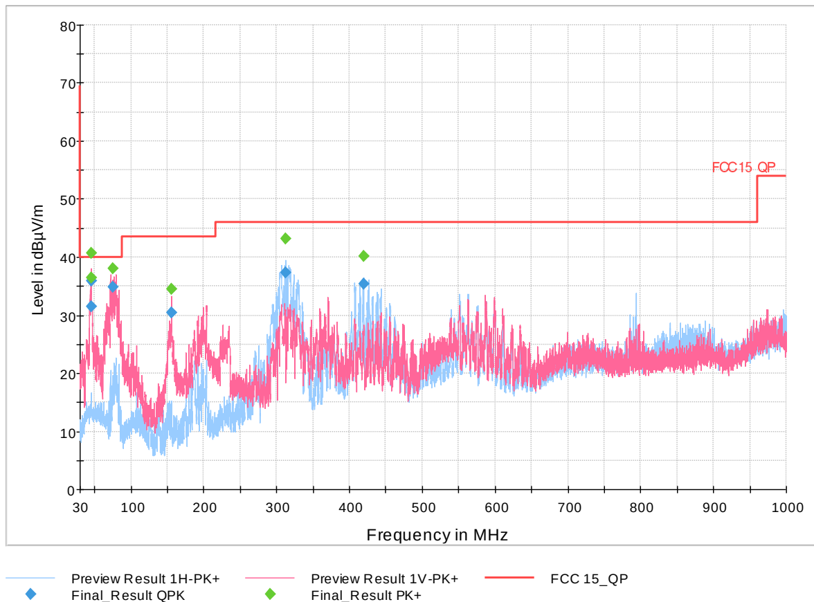
Figure 39: Radiated Spurious Emissions 30MHz – 1GHz, 2402MHz, 1Mbps
