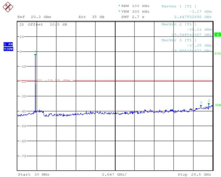
Figure 32: Conducted Emissions, 2480 MHz, 1Mbps
