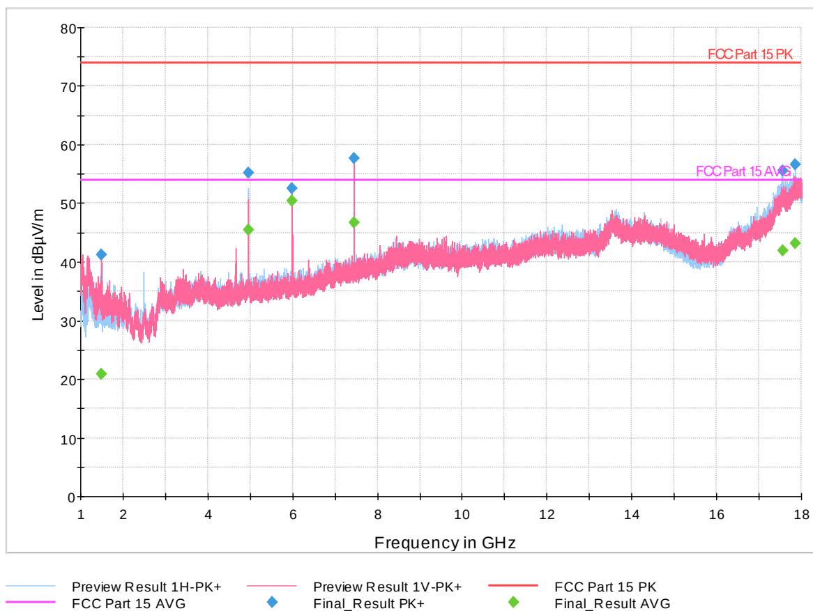
Figure 44: Radiated Spurious Emissions 1GHz - 18GHz, 2480MHz, 1Mbps
