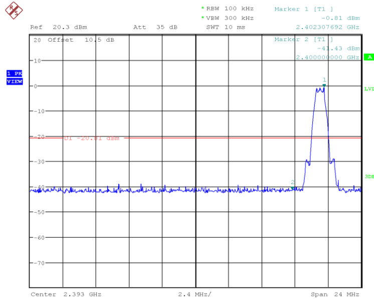
Figure 25: 2402MHz, 1Mbps, Lower Band Edge
