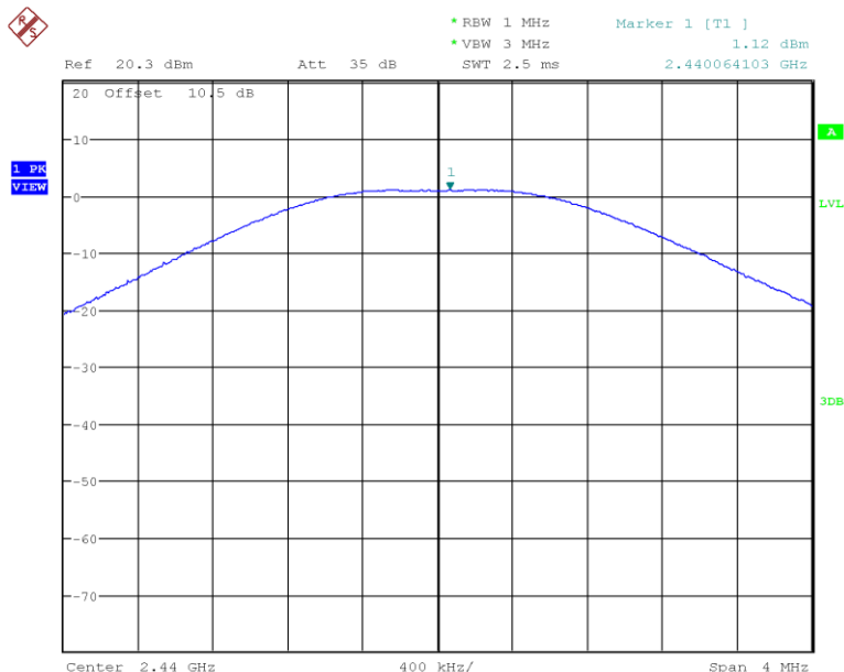
Figure 2: Maximum Conducted Power, 2440MHz, 1Mbps
