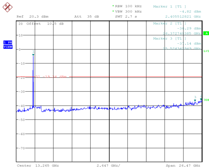
Figure 34: Conducted Emissions, 2402 MHz, 2Mbps
