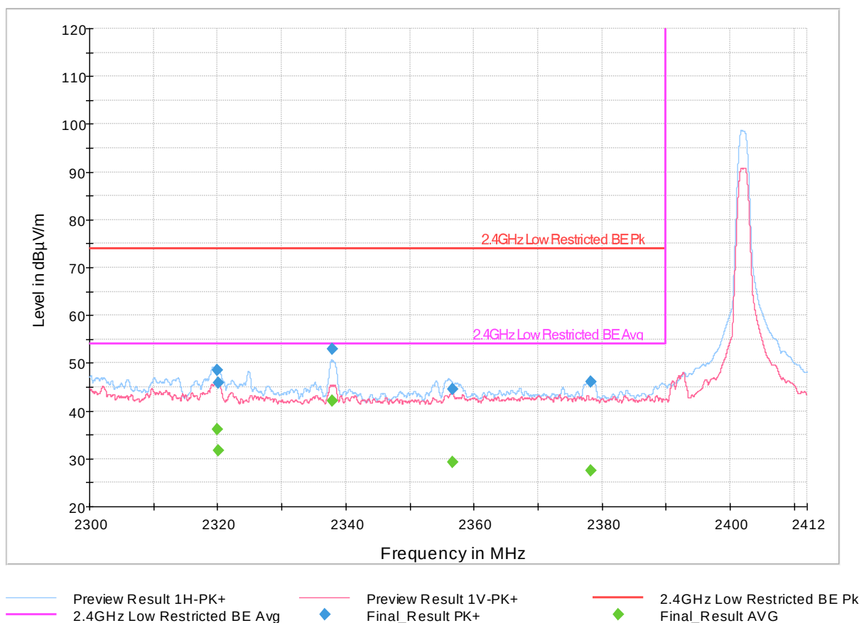
Figure 37: Restricted Band Edge, Low, 2402MHz, 1 Mbps
