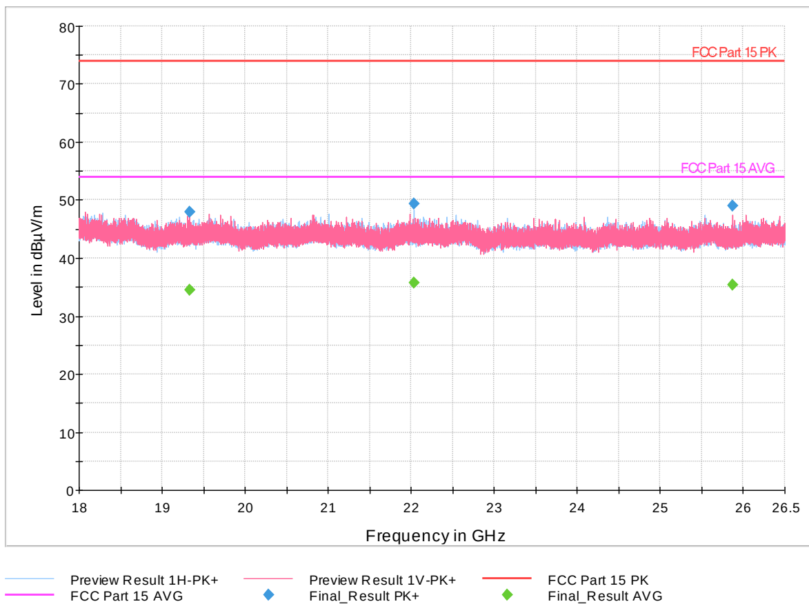
Figure 46: Radiated Spurious Emissions 18GHz - 26GHz, 2440MHz, 1Mbps
