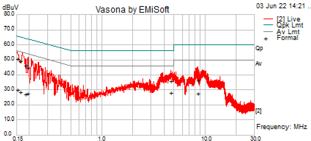
Figure 48: AC Conducted Emissions 150 kHz to 30 MHz-Live Line
