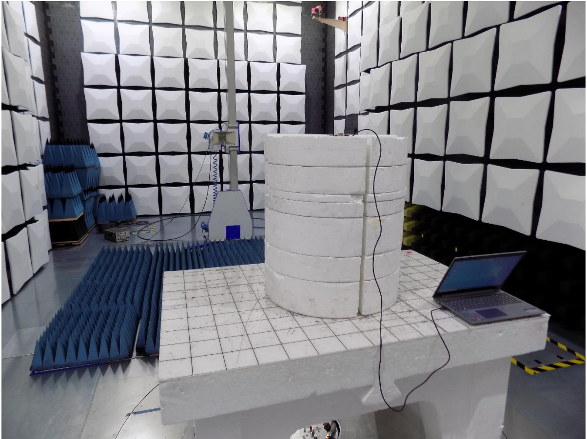
Figure 6: Test Setup for Radiated Emissions 1-18GHz - Rear View
