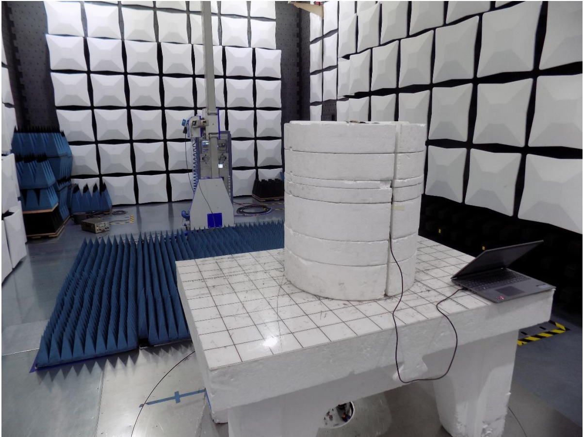
Figure 8: Test Setup for Radiated Emissions 18-26.5GHz - Rear View
