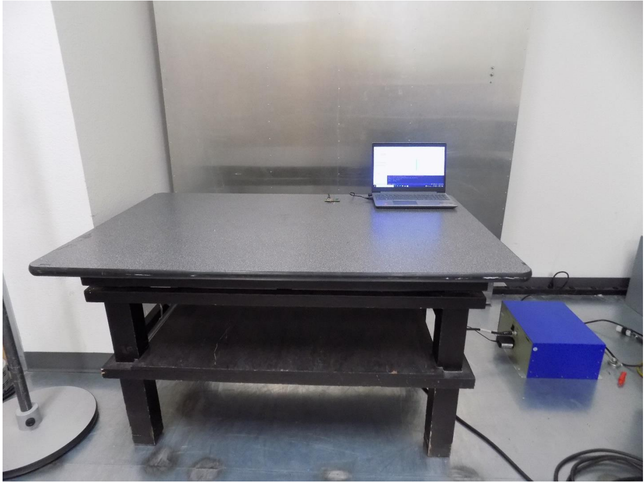
Figure 1: Test Setup for Conducted Emission – Front View
