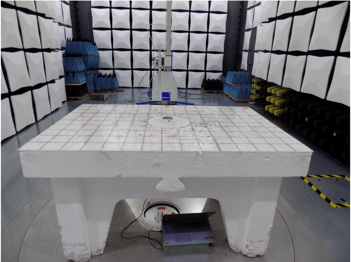
Figure 4: Test Setup for Radiated Emissions 30MHz to 1000MHz - Rear View
