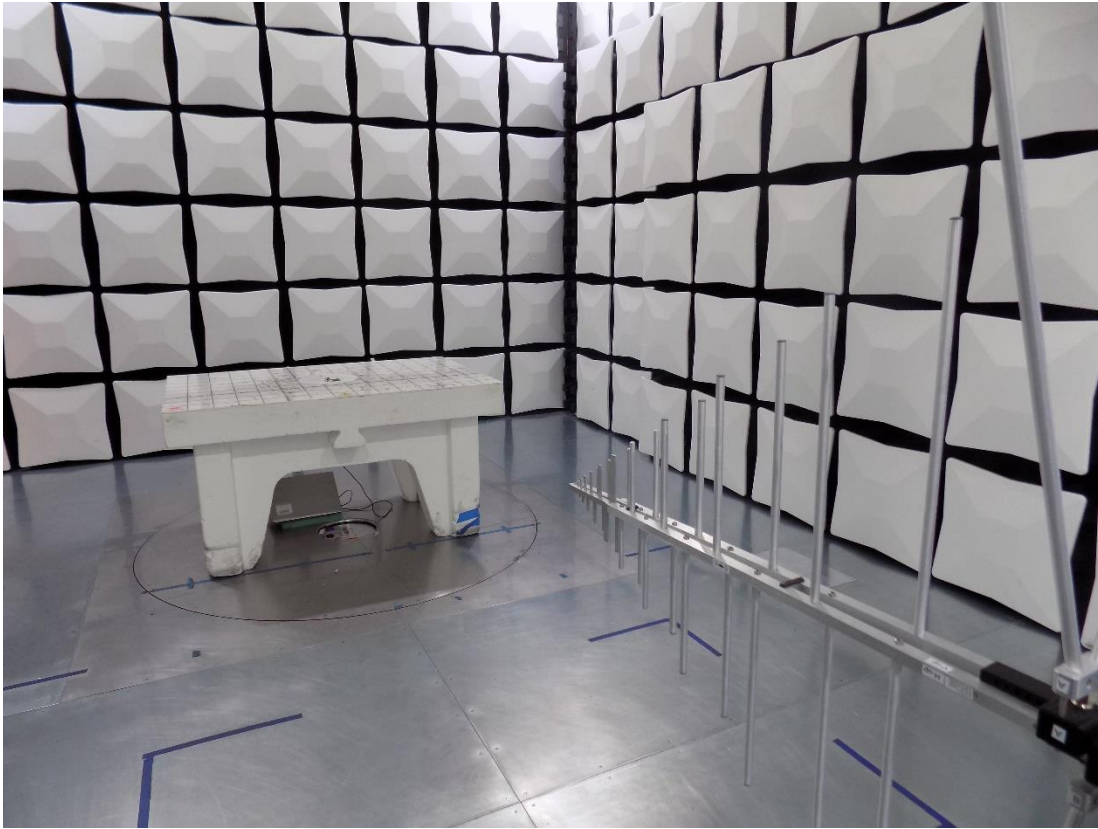
Figure 3: Test Setup for Radiated Emissions 30MHz to 1000MHz - Front View
