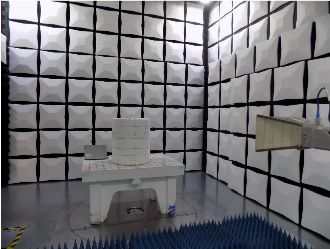
Figure 5: Test Setup for Radiated Emissions 1-18GHz - Front View
