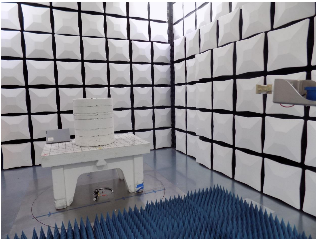
Figure 7: Test Setup for Radiated Emissions 18-26.5GHz - Front View
