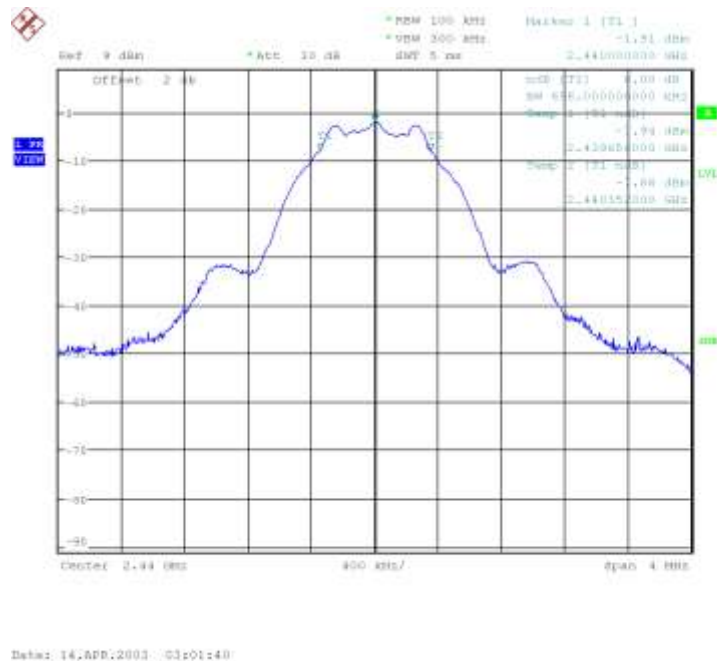
Plot 5. 2440MHz, 1Mbps, 6dB Bandwidth
