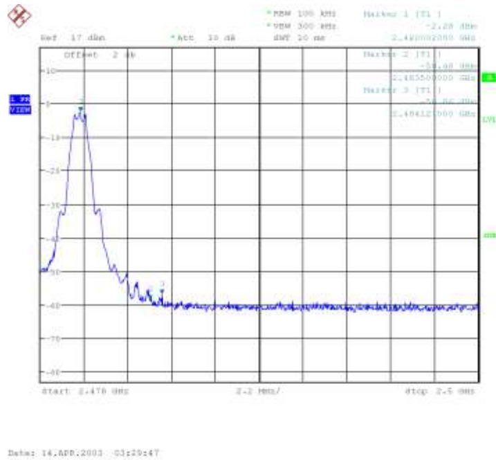
Plot 14. 2480MHz, 1Mbps Upper Band Edge
