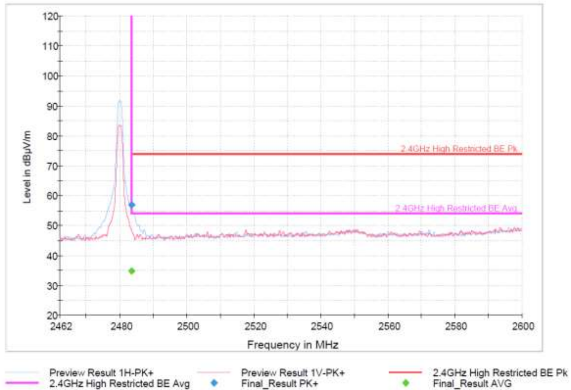
Figure 20. Upper Band Edge (Radiated) – BT BLE – 2480 MHz
