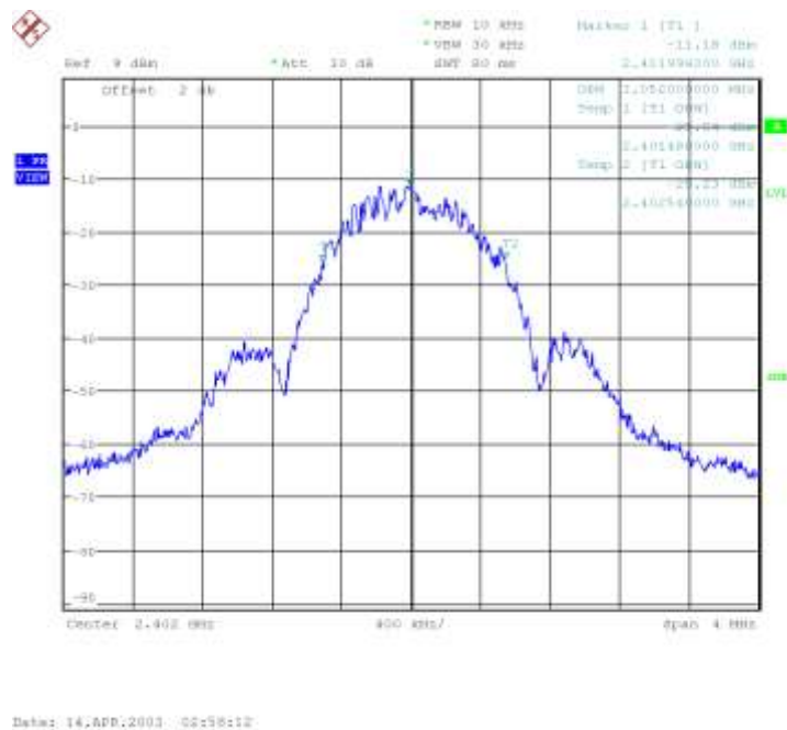
Plot 7. 2402MHz, 1Mbps, 99% Bandwidth
