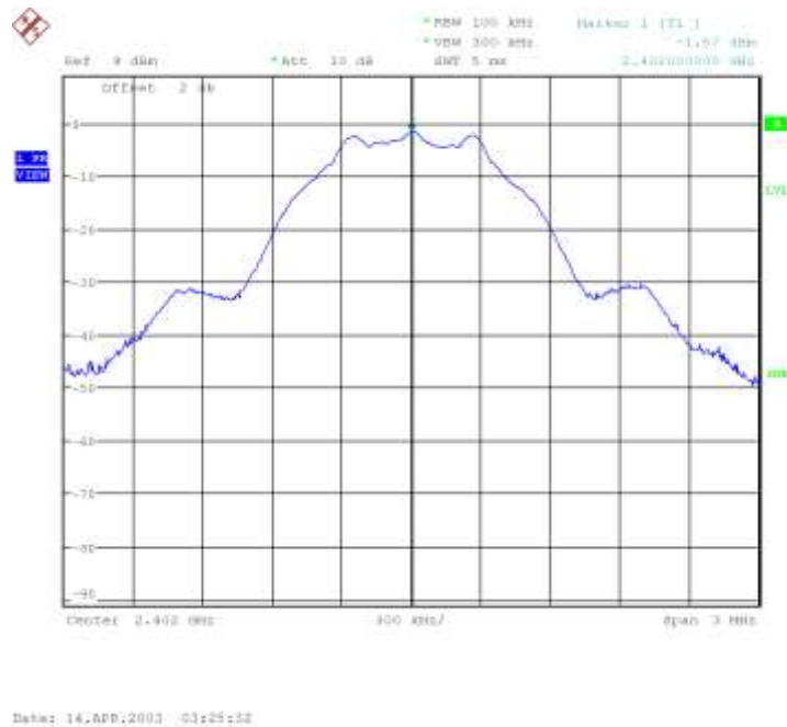
Plot 15. 1Mbps Ref Measurement
