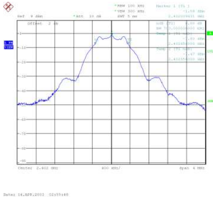
Plot 4. 2402MHz, 1Mbps, 6dB Bandwidth
