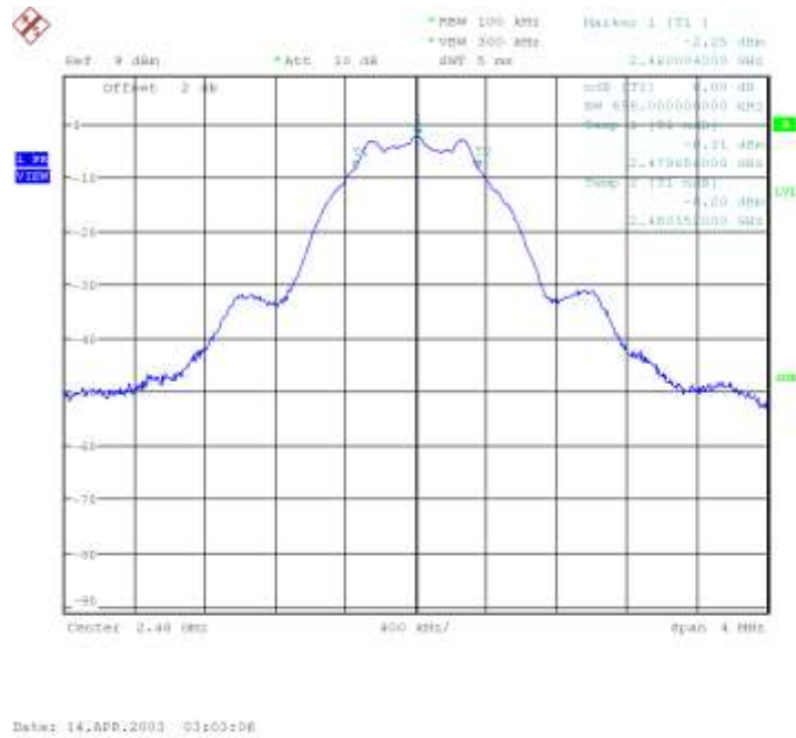
Plot 6. 2480MHz, 1Mbps, 6dB Bandwidth
