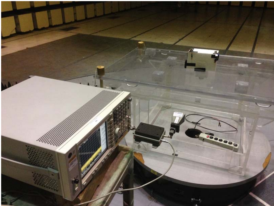
Radiated Emissions Above 18 GHz Front
