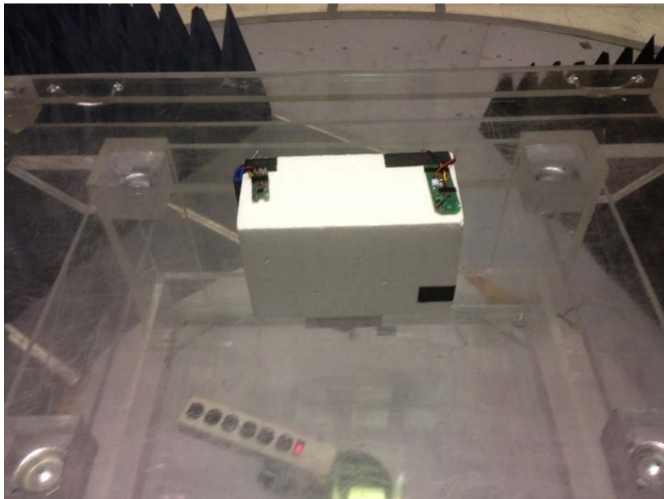
Radiated Emissions to 18 GHz Front
