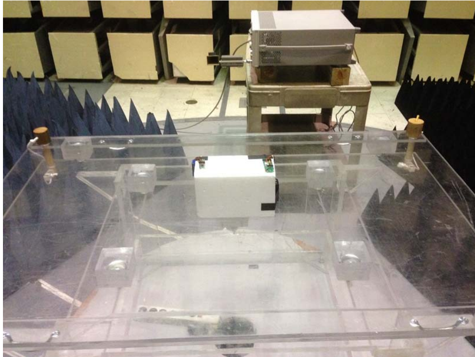
Radiated Emissions Above 18 GHz Back
