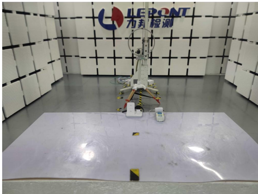
Watch wireless charger(2W)
