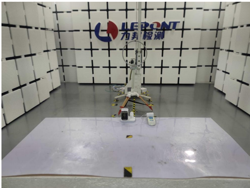
Phone wireless charger(10W)
