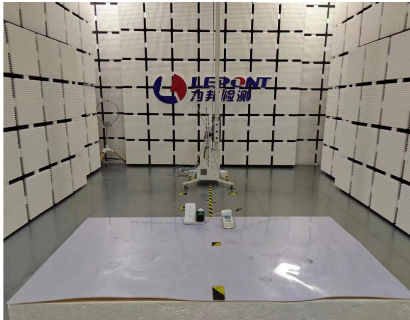
Earphone wireless charger(3W)
