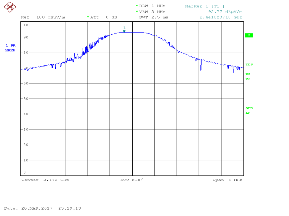
Figure 2 - 2442 MHz
