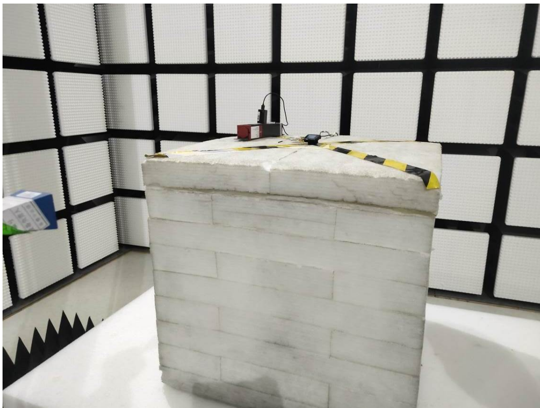
Radiated Emission Above 26.5-40GHz View
