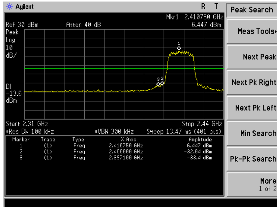
Antenna 2 802.11g: Band Edge, Left Side
