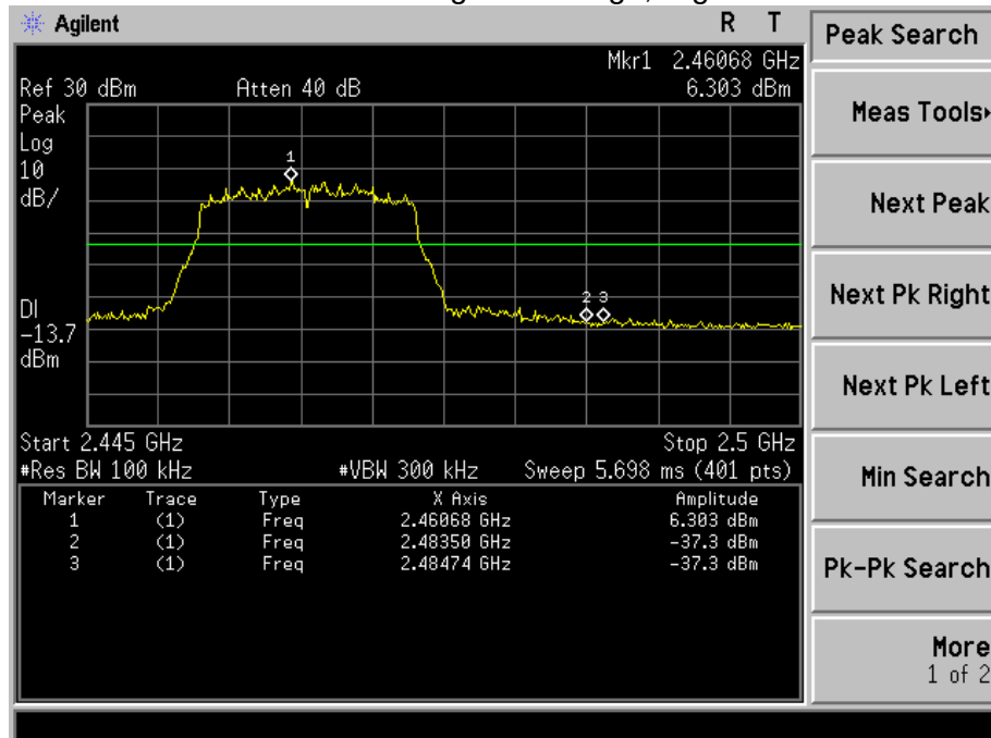
Antenna 2 802.11g: Band Edge, Right Side
