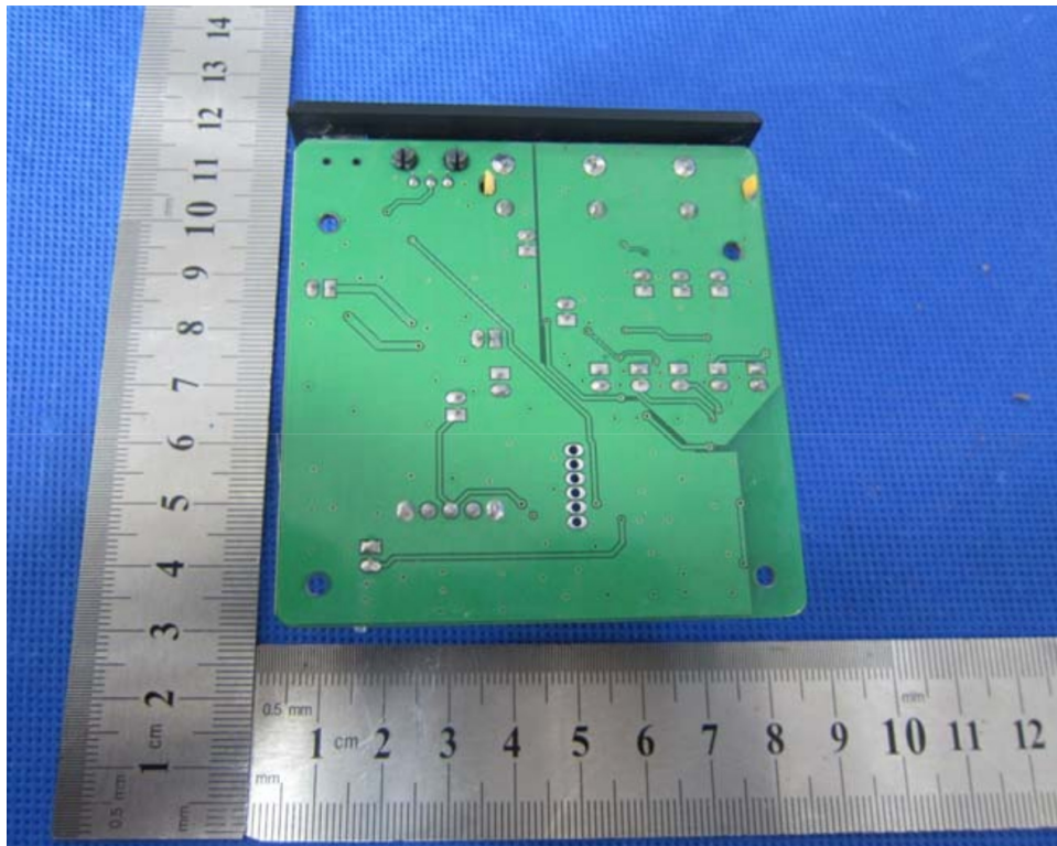
Photo 5 Appearance of PCB
