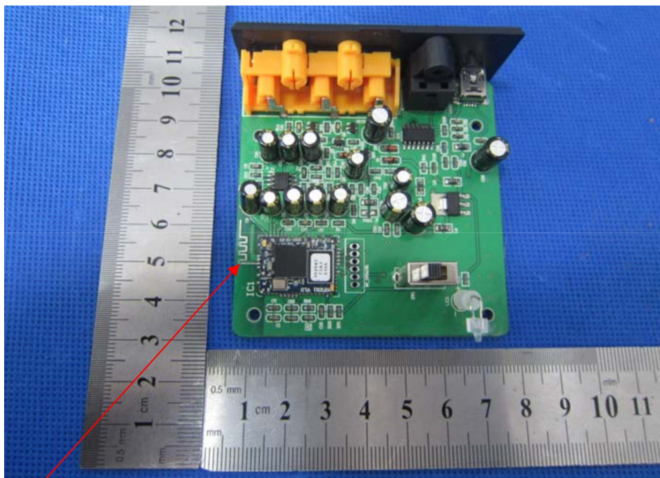
2.4G PCB Antenna
