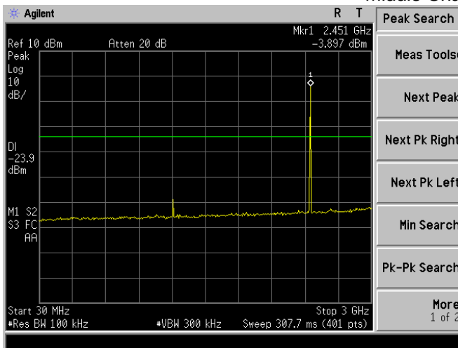
Middle Channel 2448MHz
