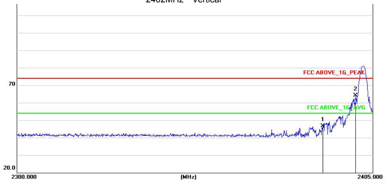
2402MHz Vertical
