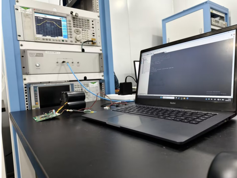
Conducted Emissions at Mains Power Port (150kHz-30MHz)
