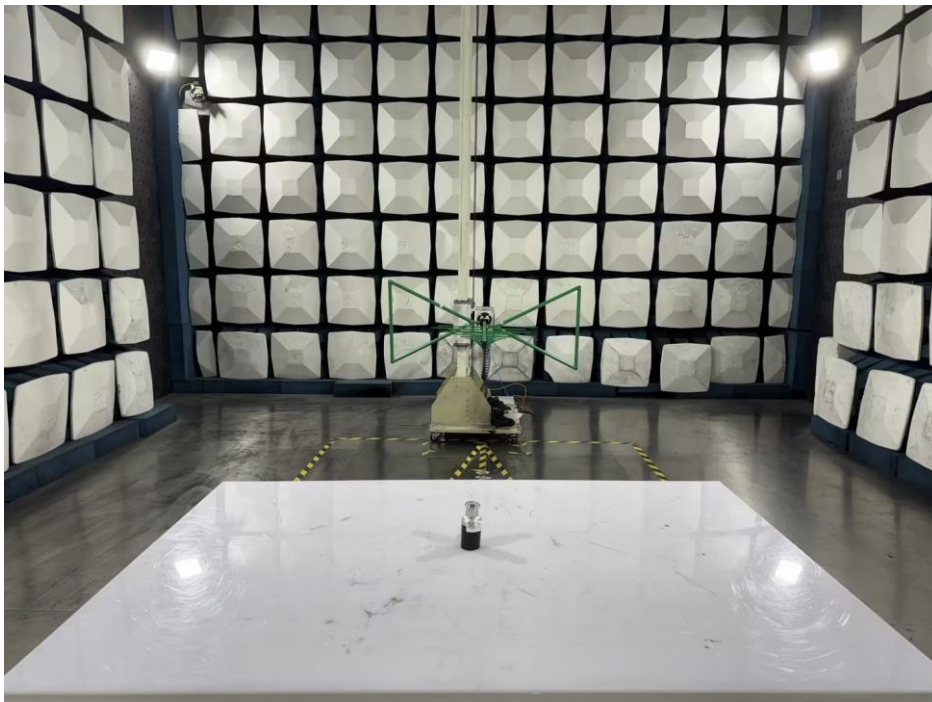
Radiated emissions spurious (Below 1GHz)
