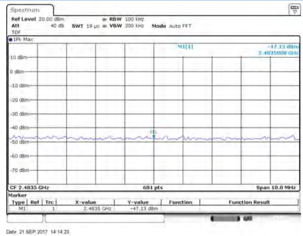
802.11n-40 MHz HIGH CHANNEL, Band Edge
