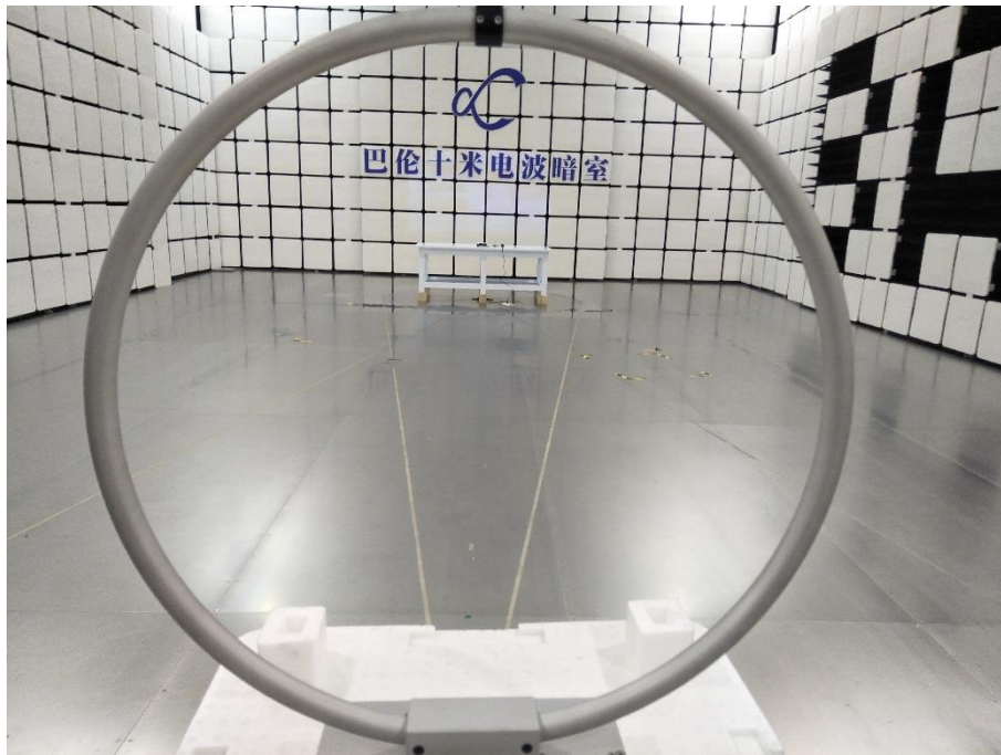
Radiated Test 1
