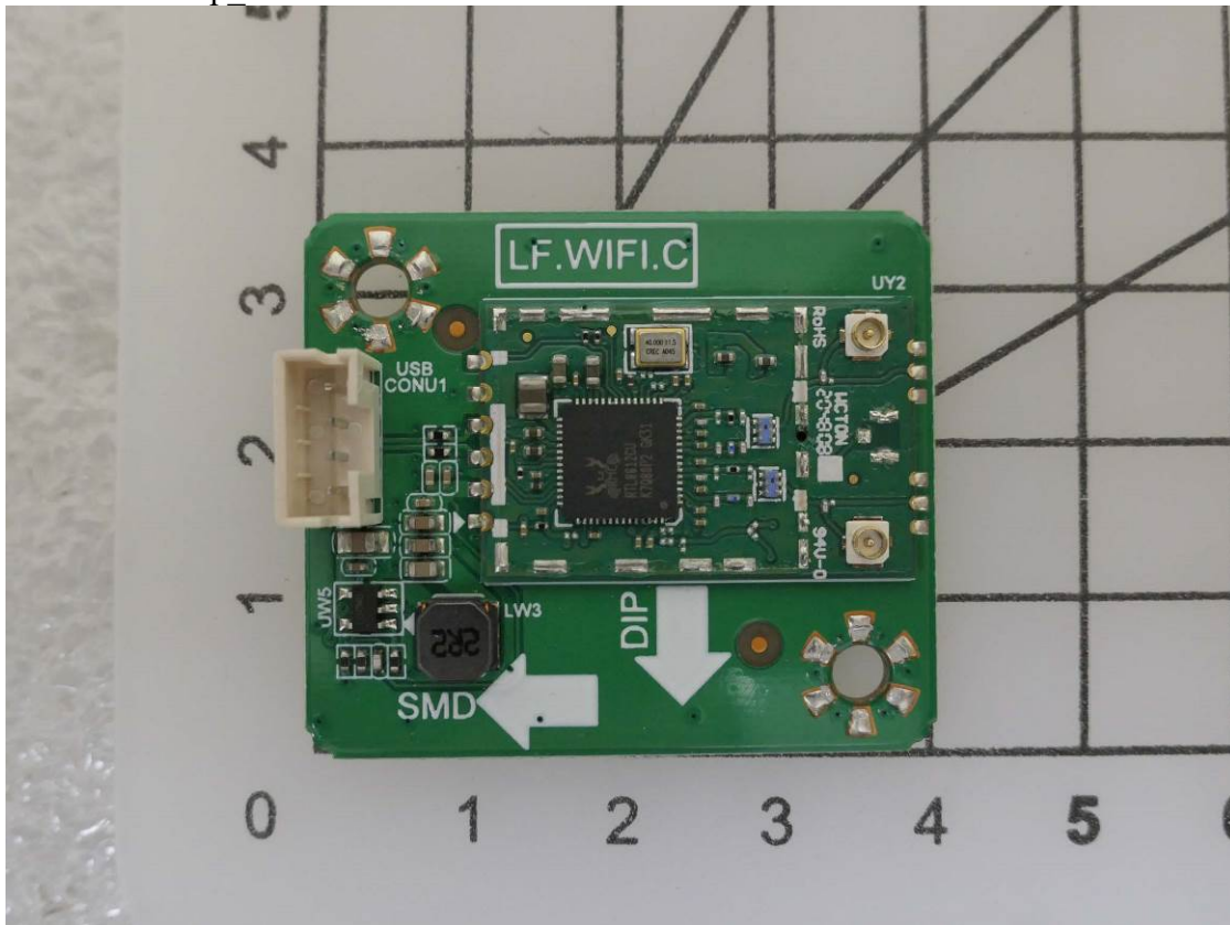
EUT-15. Chip RTL8812CU
