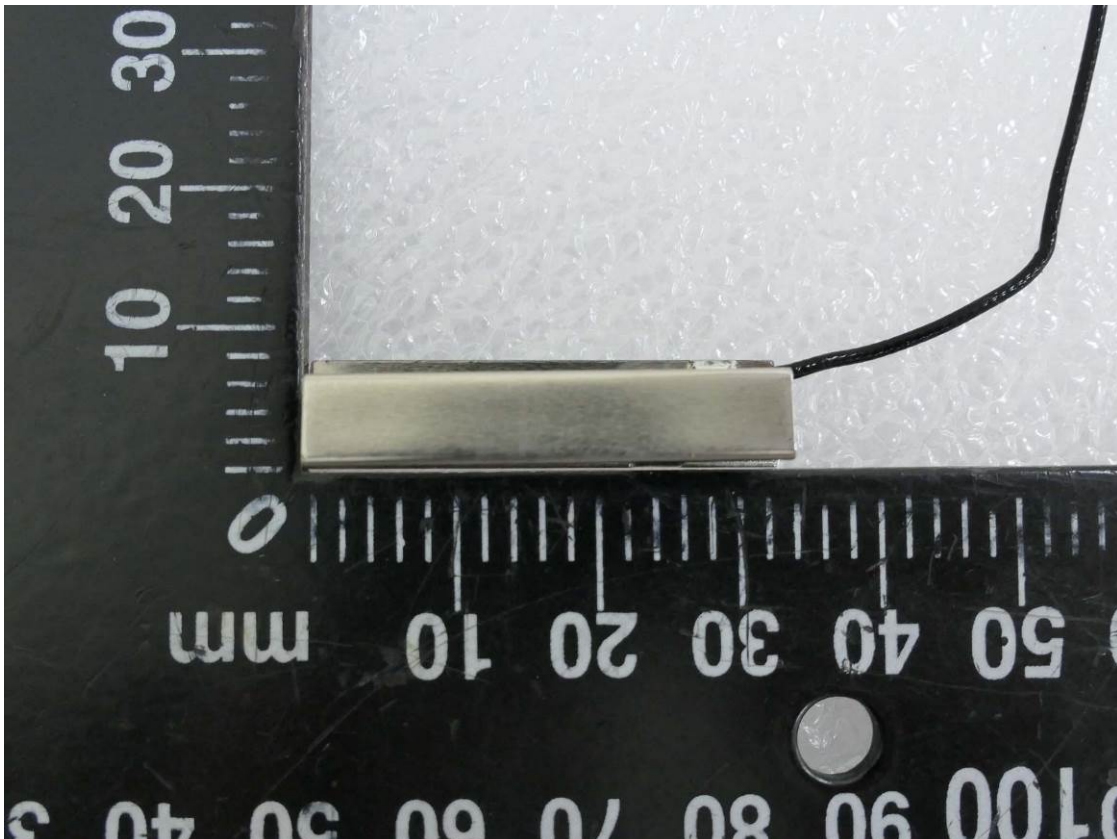
EUT-18. Antenna
