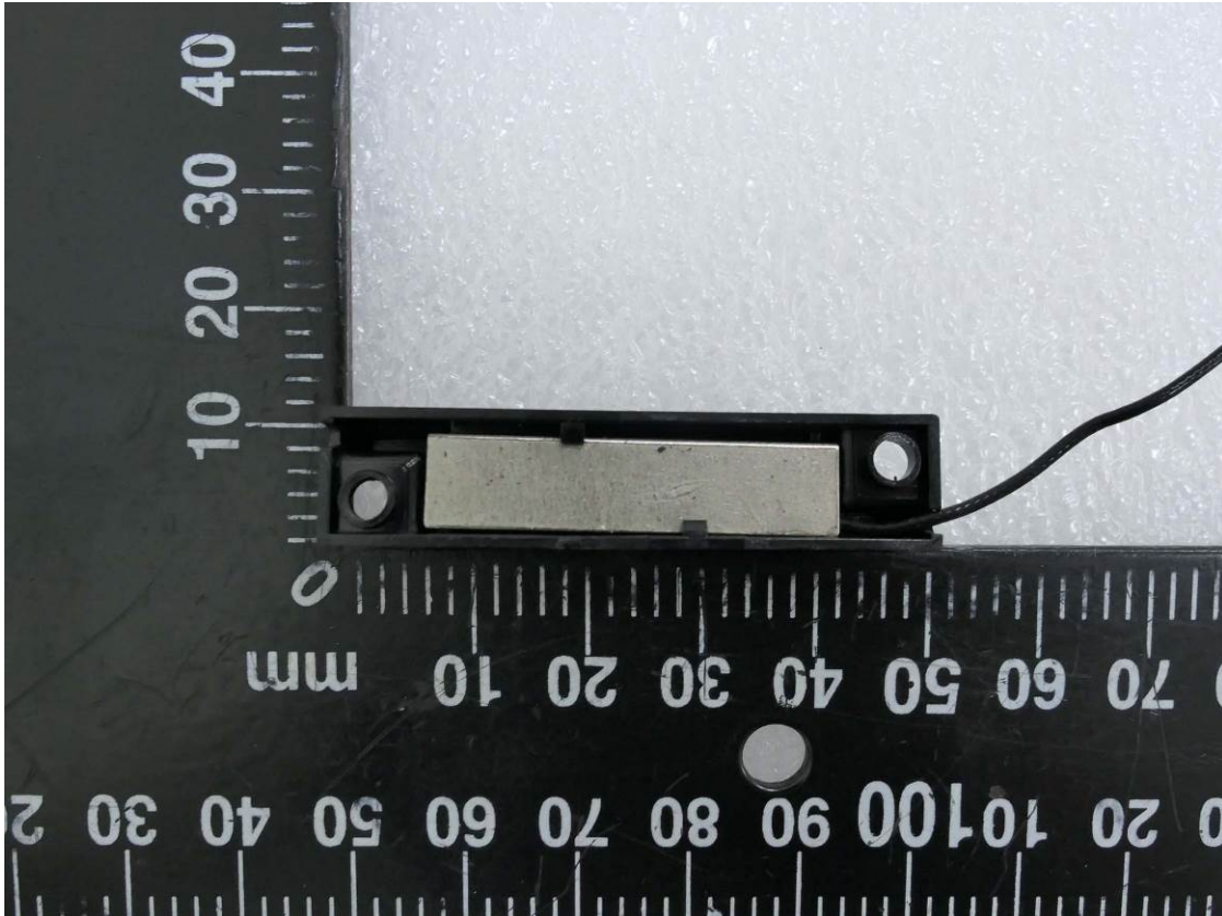
EUT-17. Antenna
