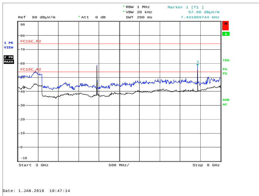
Figure 25 - 2475 MHz - 3 GHz to 8 GHz - Horizontal and Vertical
