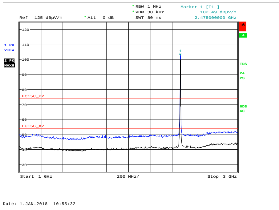
Figure 24 - 2475 MHz - 1 GHz to 3 GHz - Horizontal and Vertical
