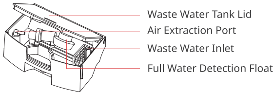
Waste Water Tank Components
