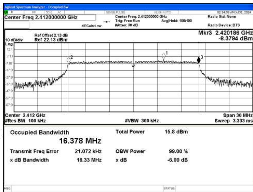
-6dB Bandwidth NVNT g 2412MHz Ant
