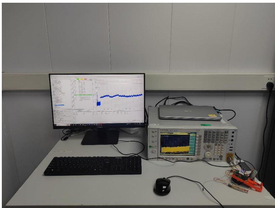
Conducted Test-BLE/WIFI
